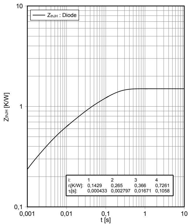
瞬态热阻抗 Diode, 转换器 transient thermal impedance Diode, Boost Z_{thJH} = f(t)
