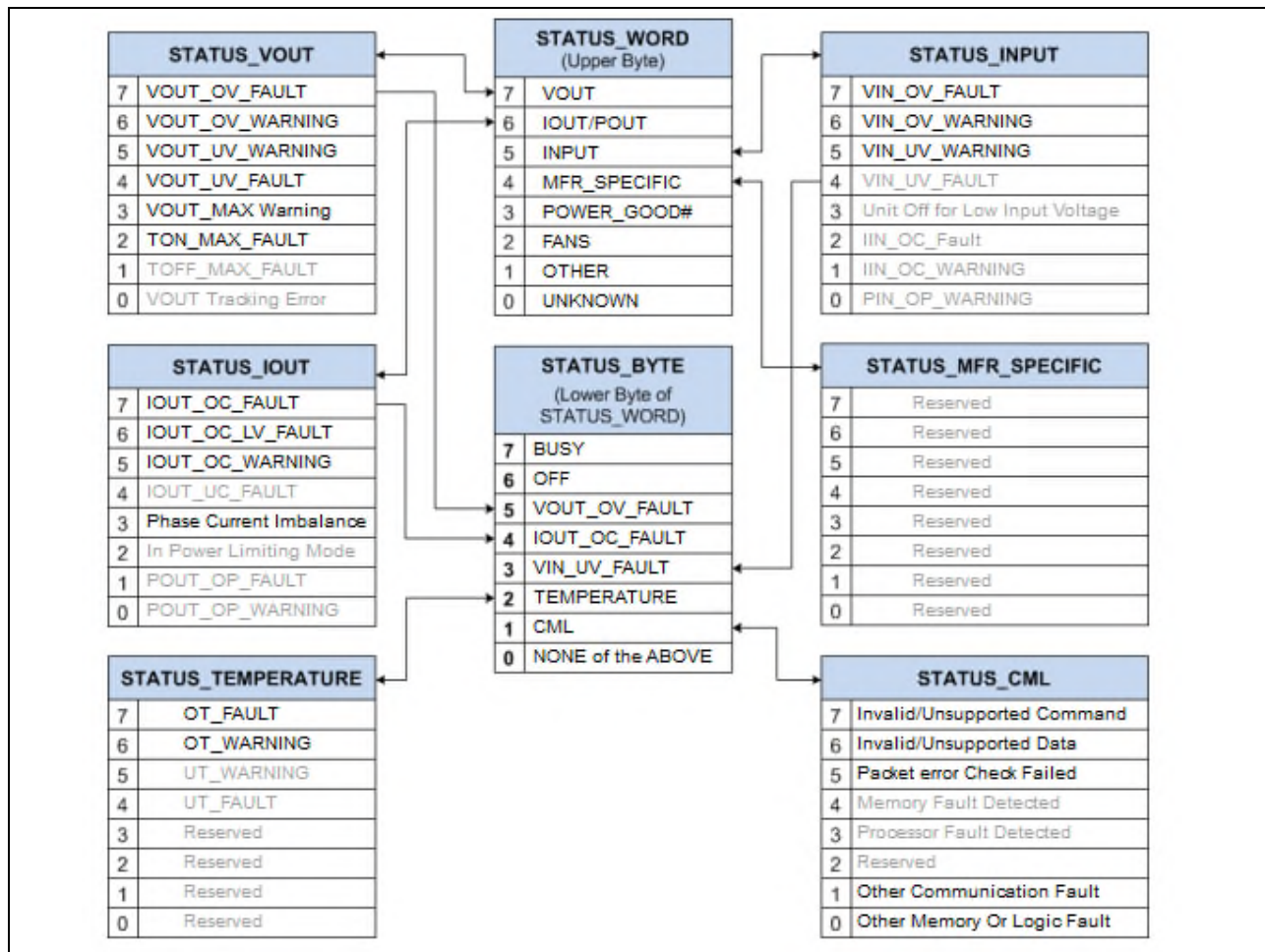
Figure 2 Active status registers for the IRPS5401
