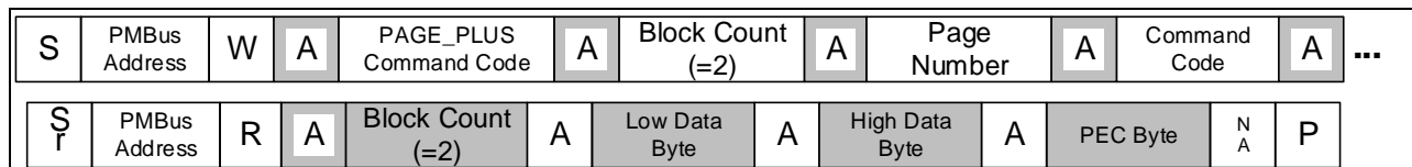
Figure 1 PAGE_PLUS_READ command example with data to read and PEC
