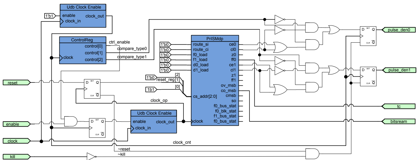
Figure 3. PrISM Implementation
