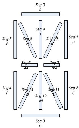
Figure 6. 14-Segment Display
