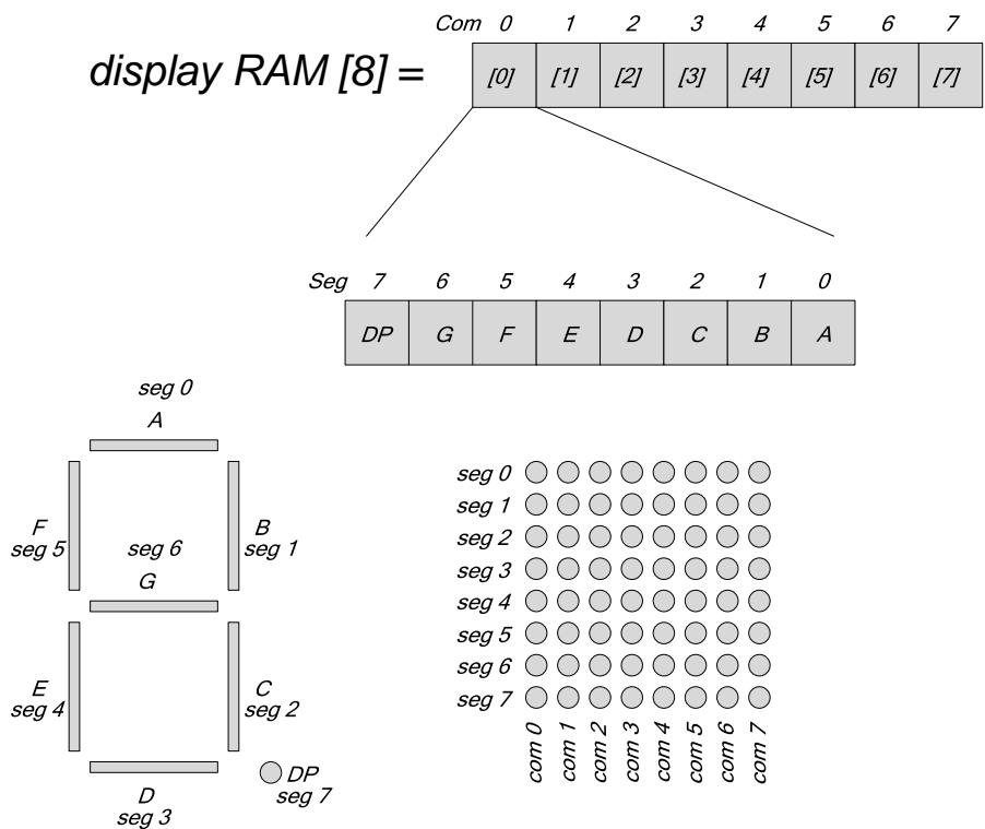
Figure 1. Display RAM
