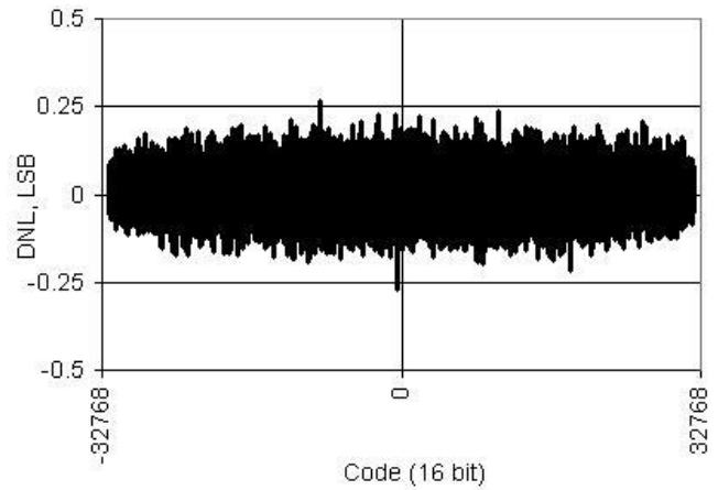
Delta-Sigma ADC DNL versus Output Code, 16-bit, 48 ksp/s, 25 °C V_{DDA} = 3.3 V
