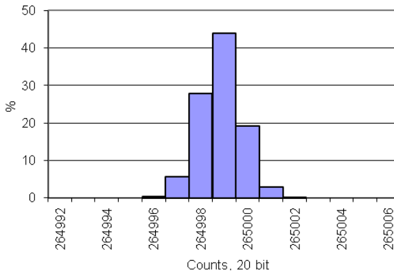
Delta-Sigma ADC Noise Histogram, 1000 Samples, 20-Bit, 187 sps, Ext Ref, V IN = V REF /2, Range = ±1.024 V
