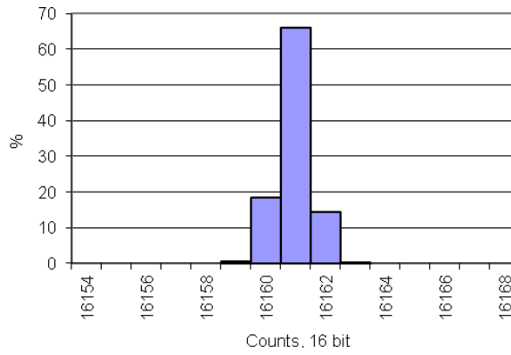
Delta-Sigma ADC Noise Histogram, 1000 samples, 16-bit, 48 kpsps, Ext Ref, V IN = V REF /2, Range = ±1.024 V
