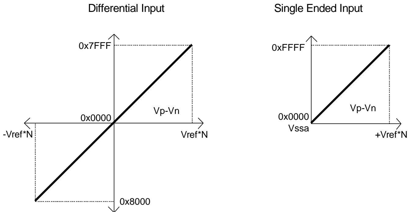
Figure 6. Delta-Sigma ADC I/O Characteristics
