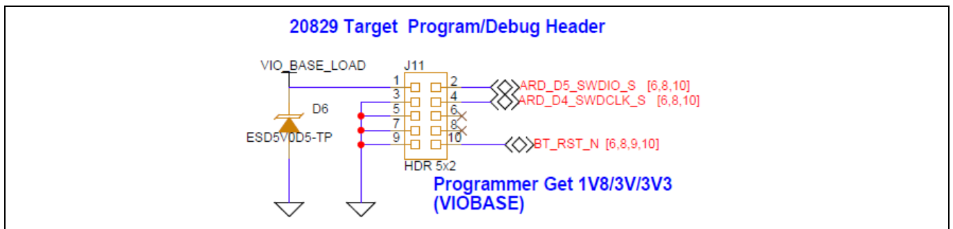
Figure 34 10-pin SWD programming/debug header
