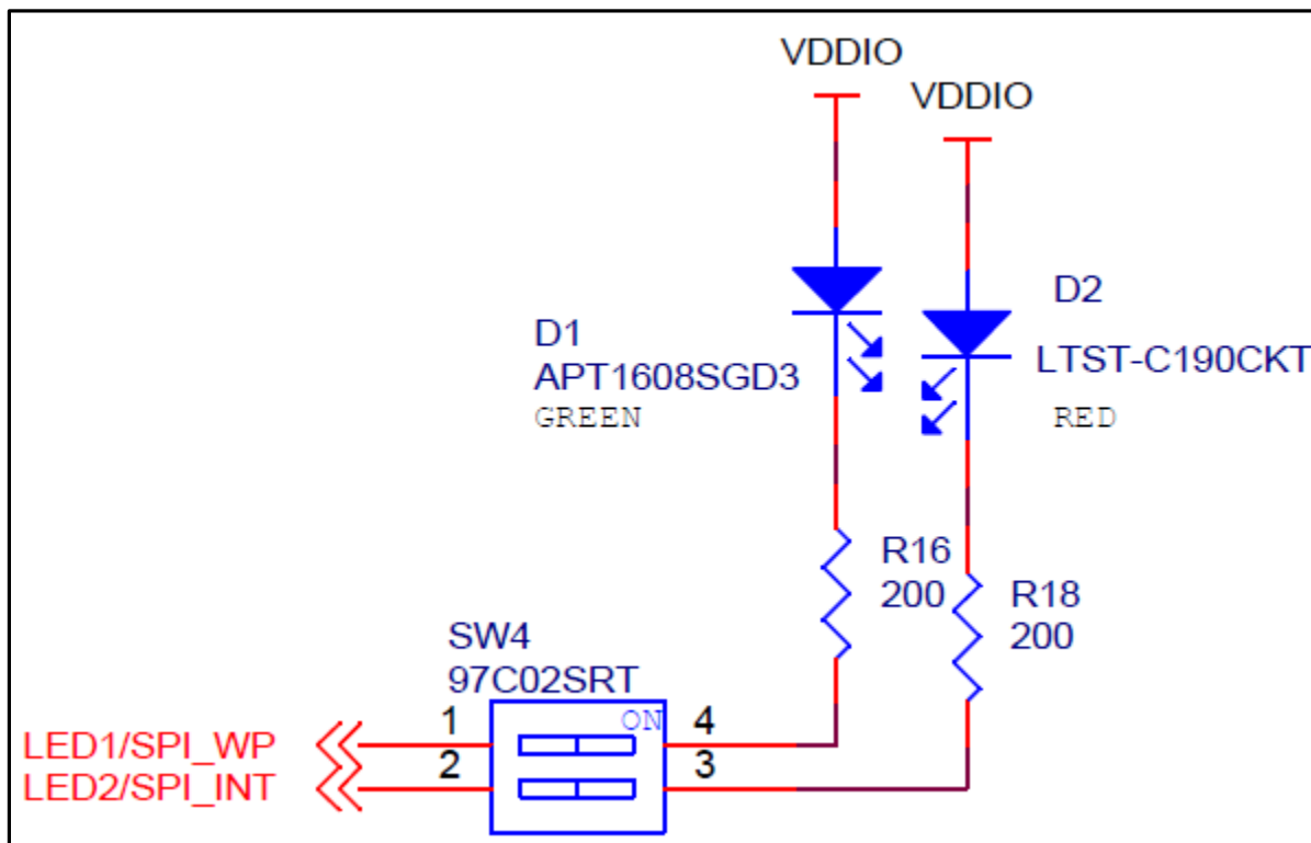
Figure 5-12. LED Circuit
