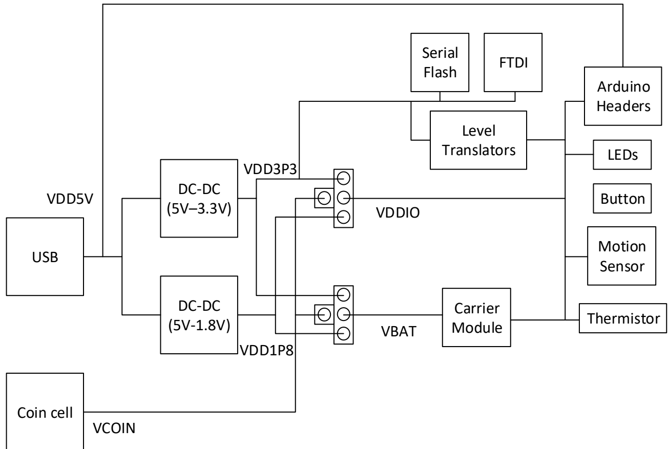
Figure 5-1. Power Architecture
