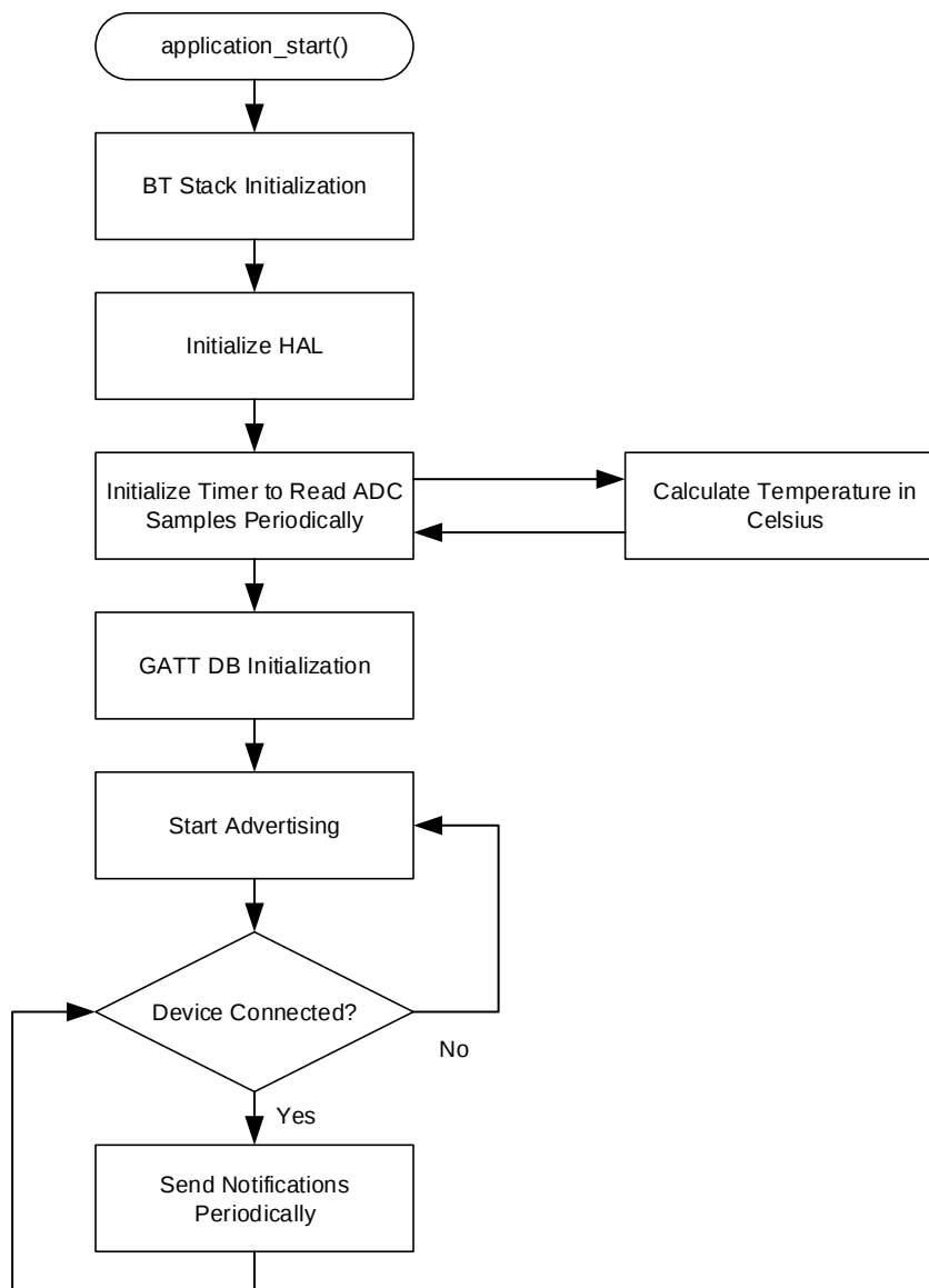
Figure 4-1. thermistor_app Flowchart
