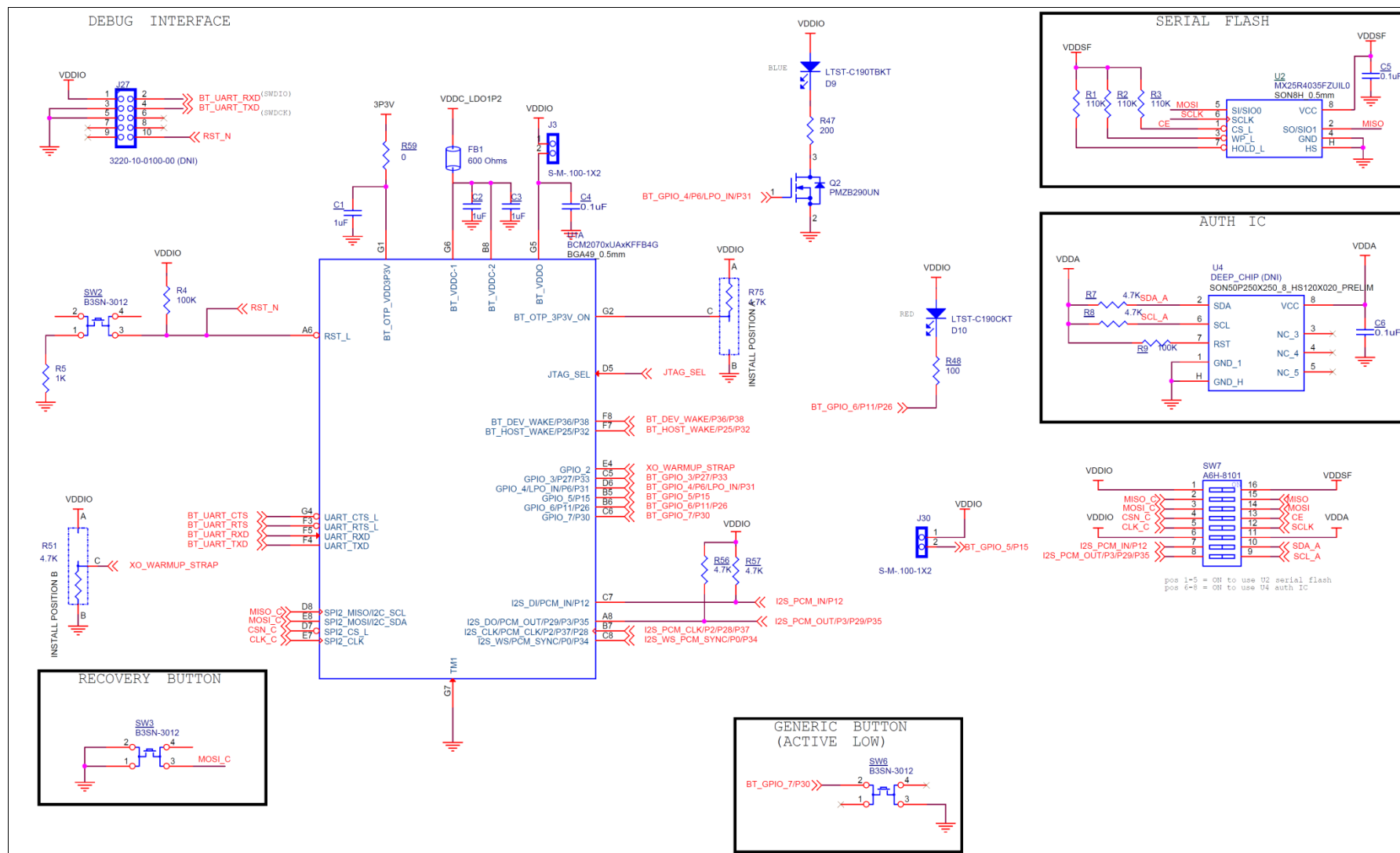
Figure 6-1. CYW920706WCDEVAL Baseband Schematic
