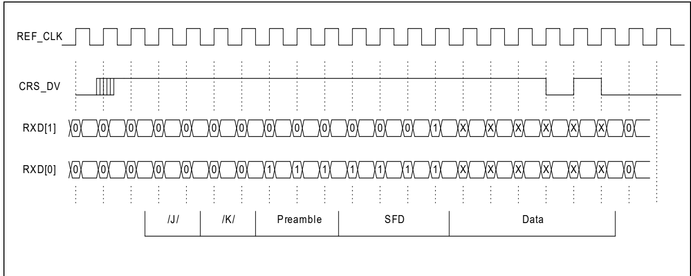
Figure 17. RMII Receive Packet Timing
