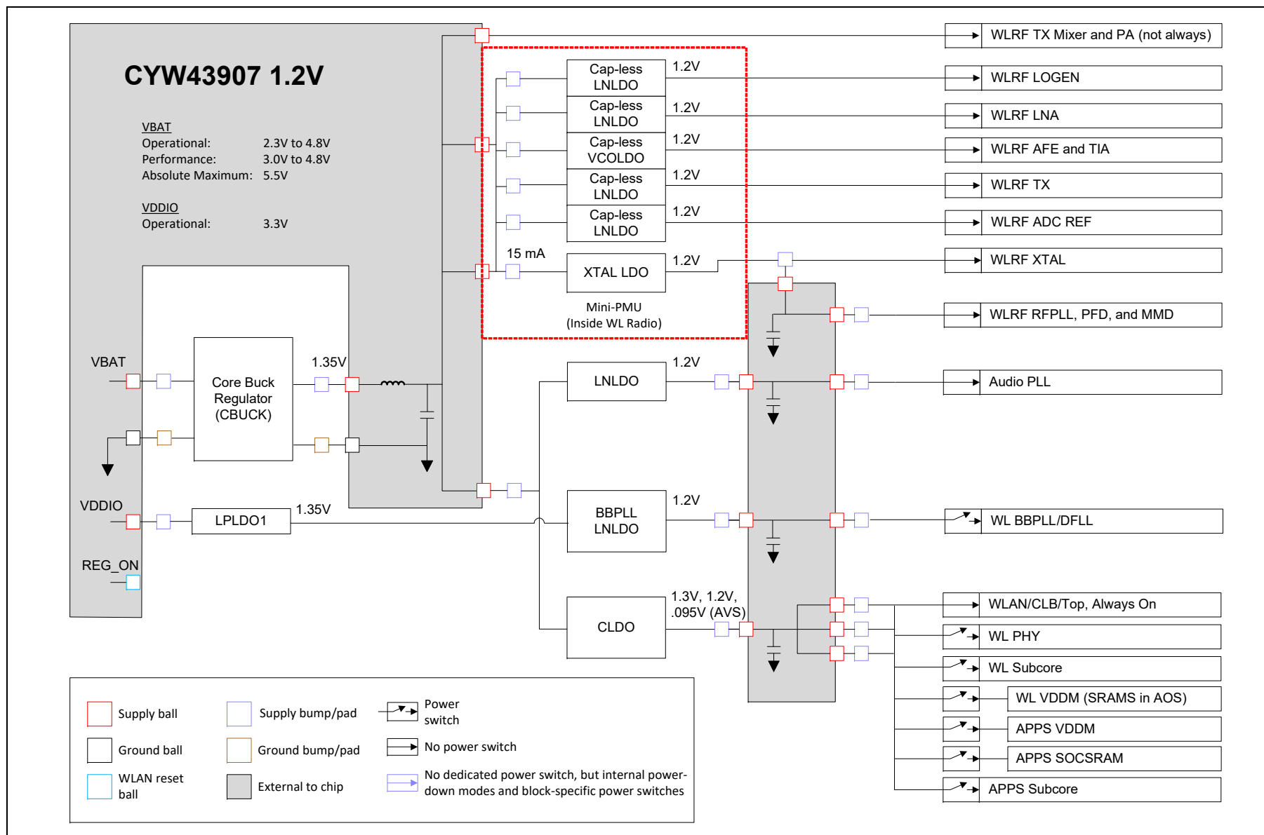
Figure 3. Typical Power Topology (Page 1 of 2)
