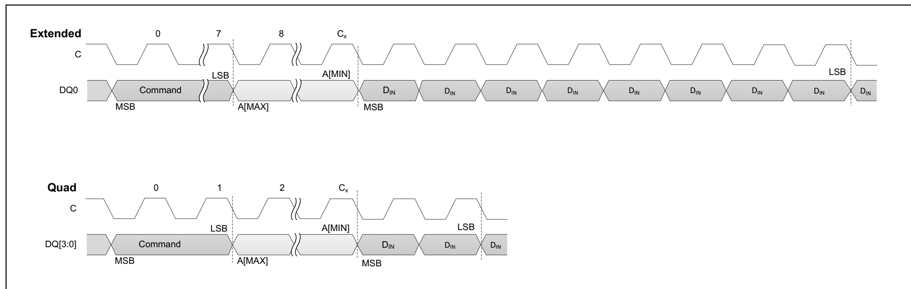
Figure 32. Memory-Write Timing
