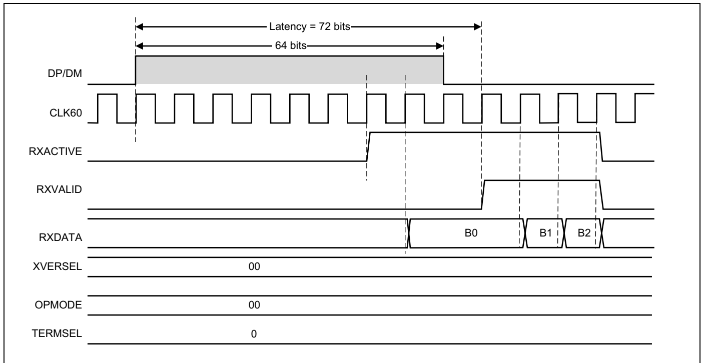
Figure 36. USB 2.0 HS Mode Receive Timing
