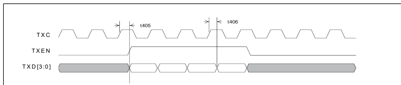
Figure 16. MII Transmit Packet Timing
