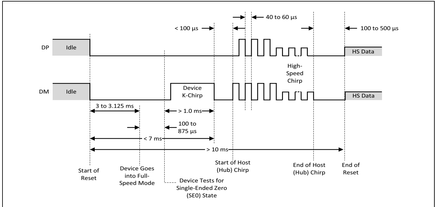
Figure 34. USB 2.0 Bus Reset to HS Mode Operation
