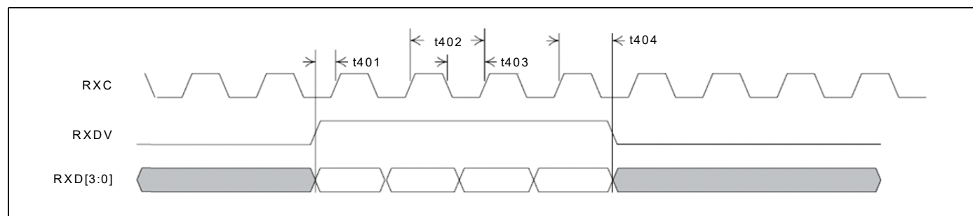
Figure 15. MII Receive Packet Timing
