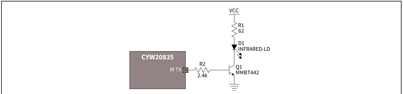
Figure 7 Infrared TX
