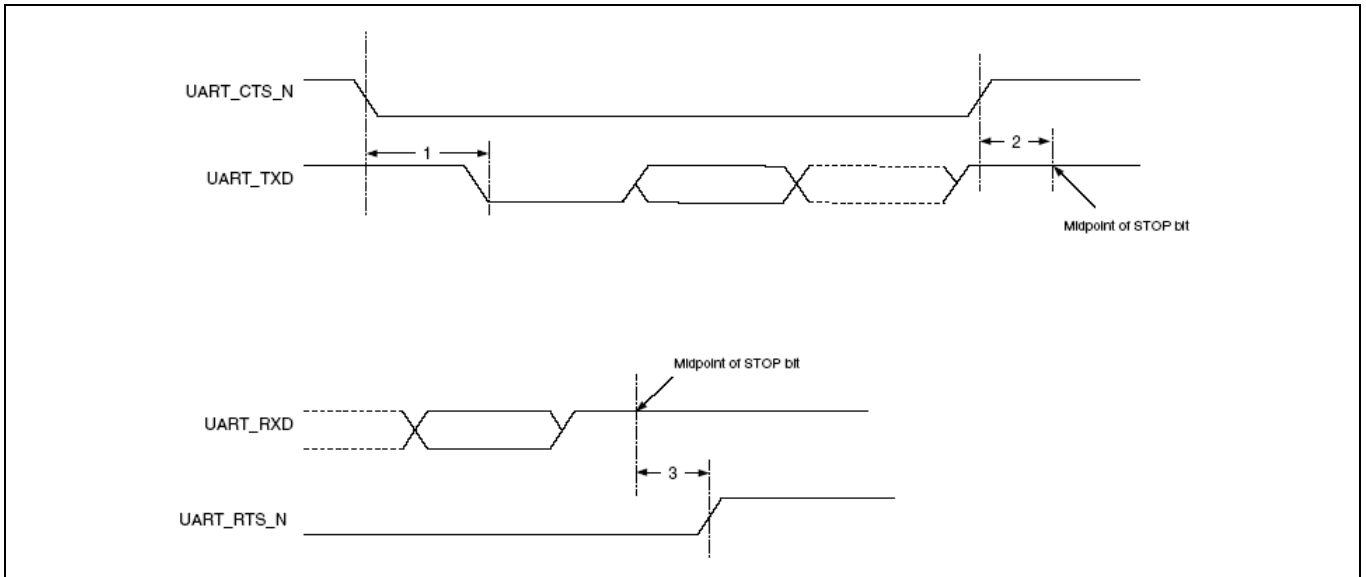
Figure 9 UART timing
