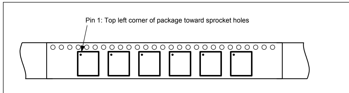
Figure 20. Pin 1 Orientation
