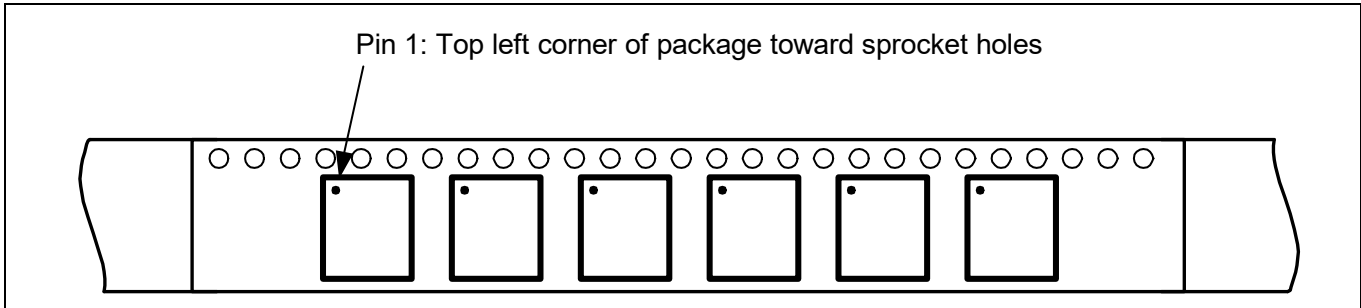
Figure 17 Pin 1 orientation
