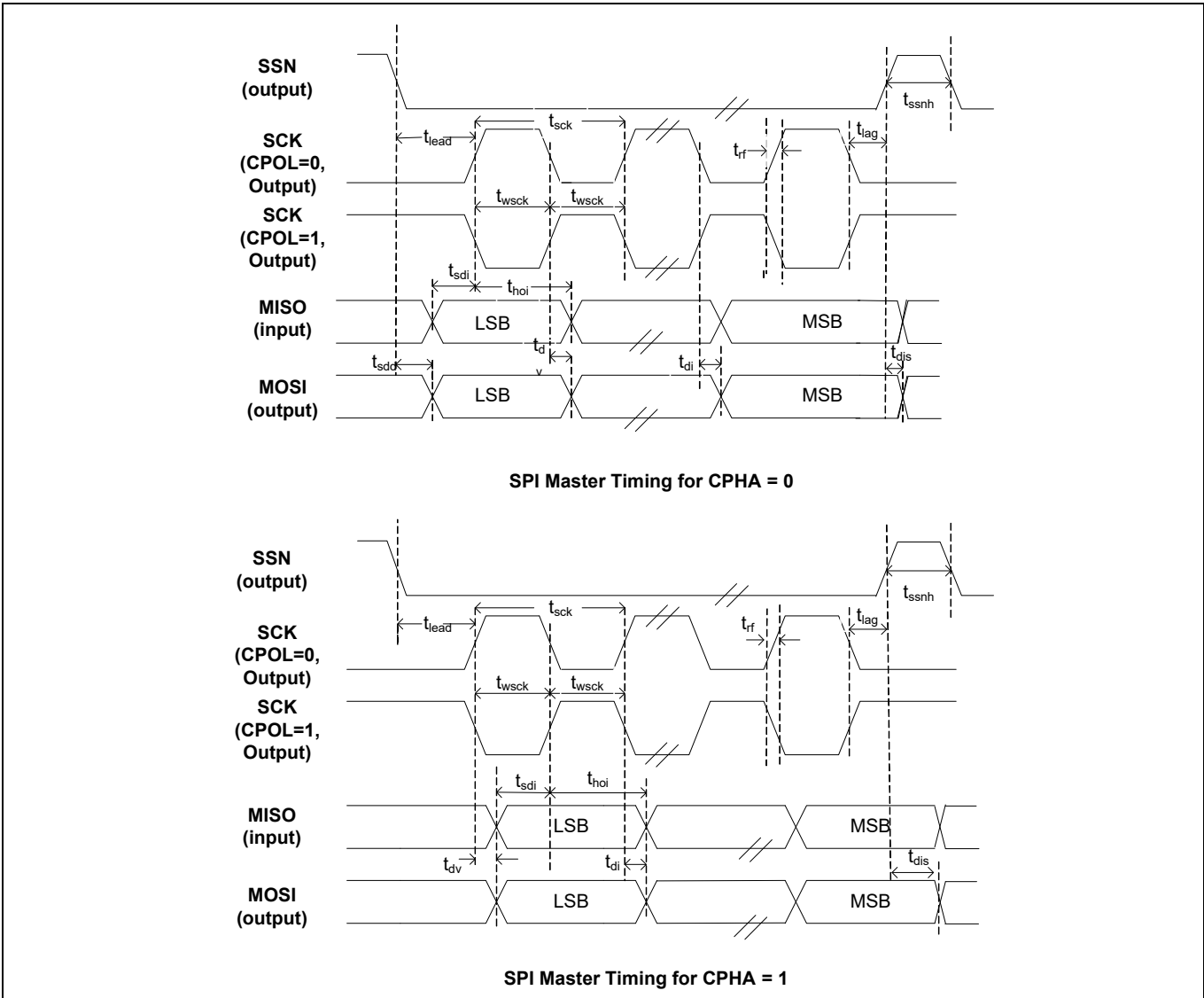
Figure 10 SPI timing
