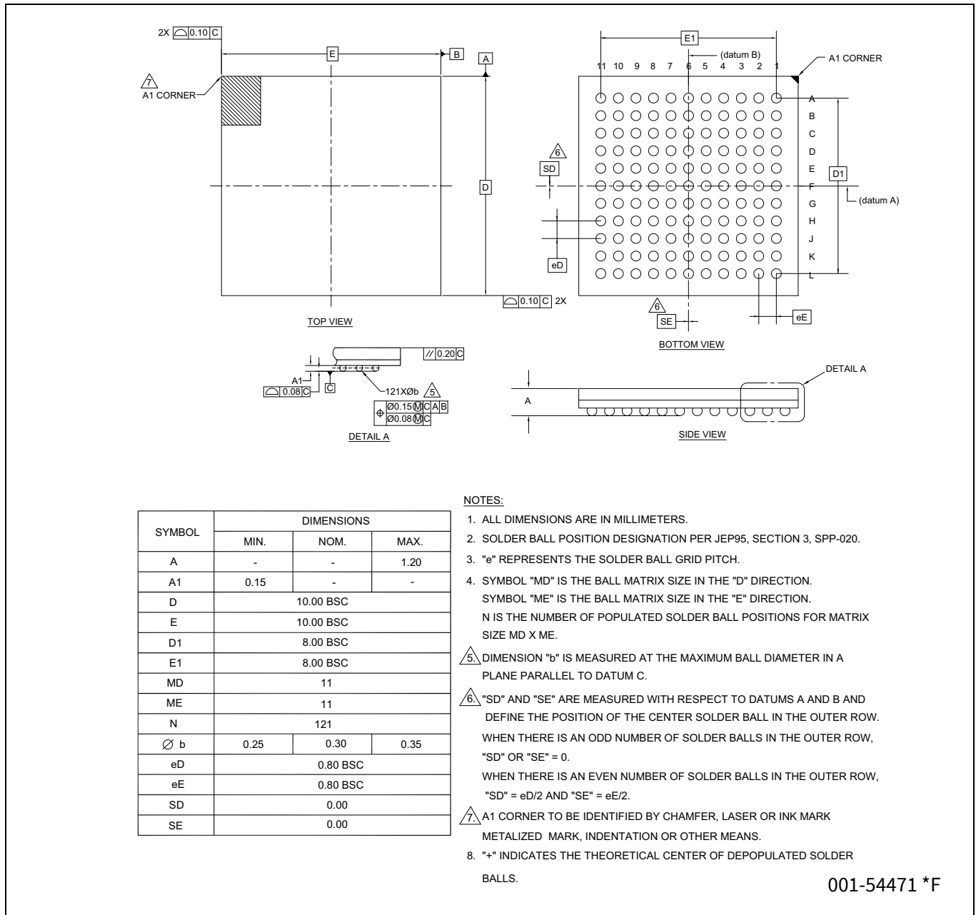
Figure 7 121-ball FBGA (10 x 10 x 1.20 mm) package outline, 001-54471
