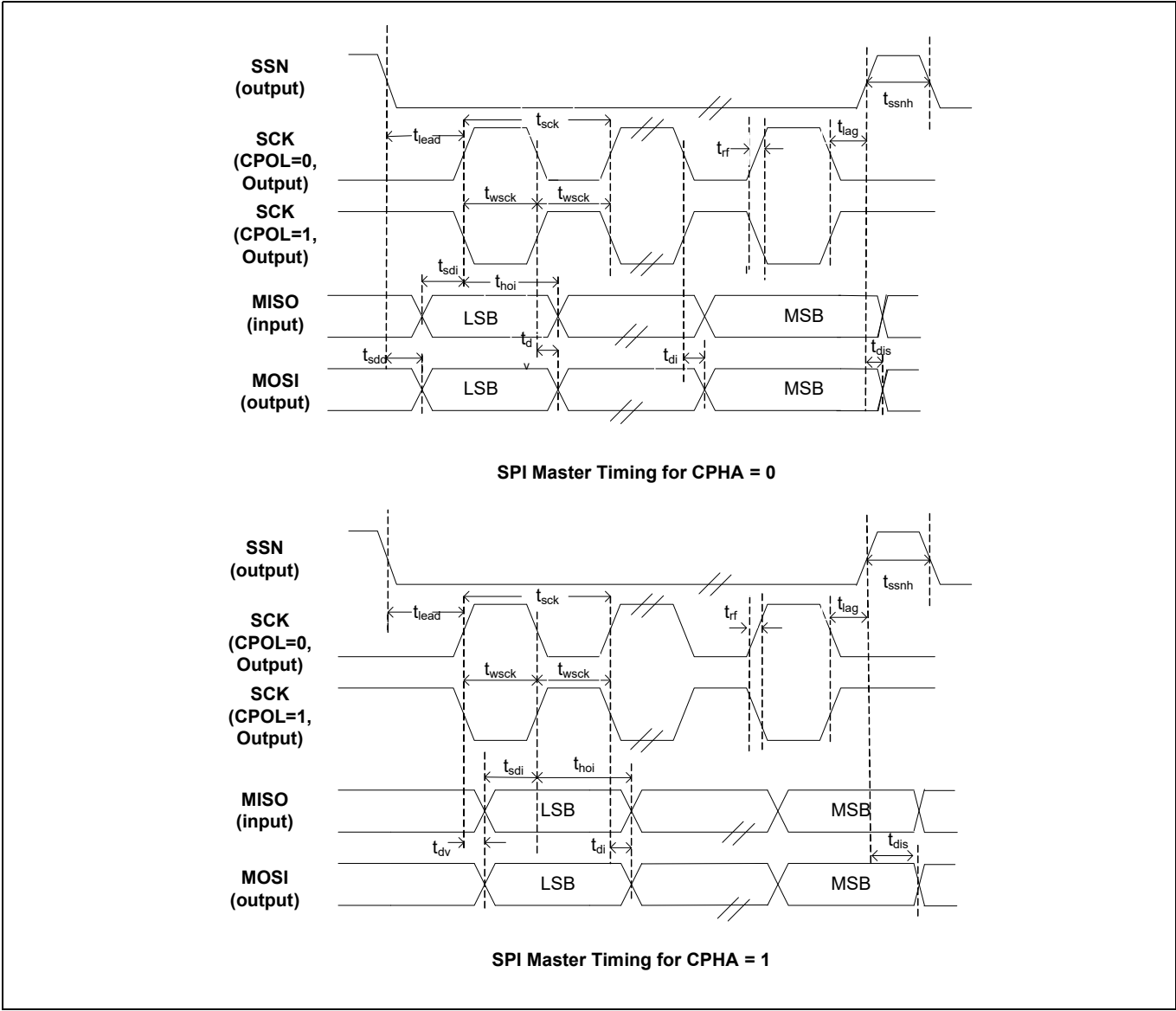
Figure 5 SPI timing
