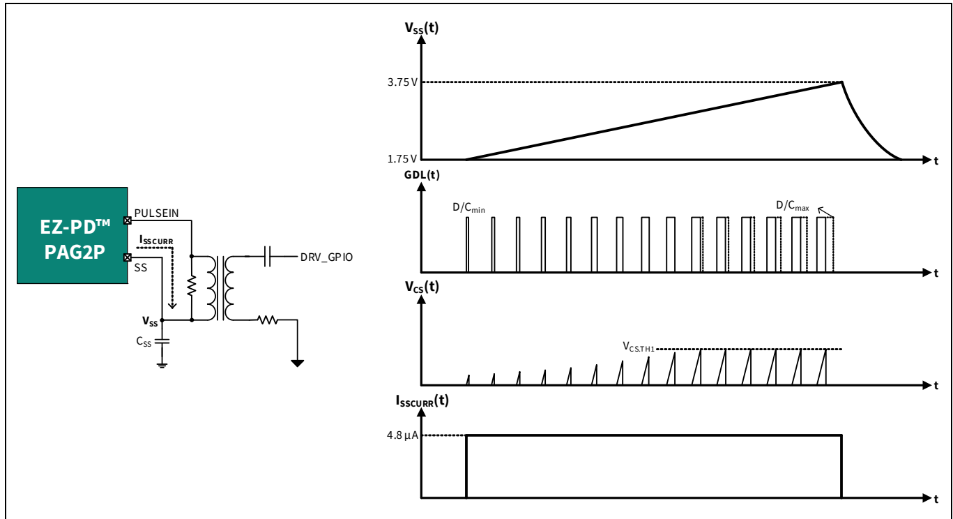
Figure 5 Soft-start operation
