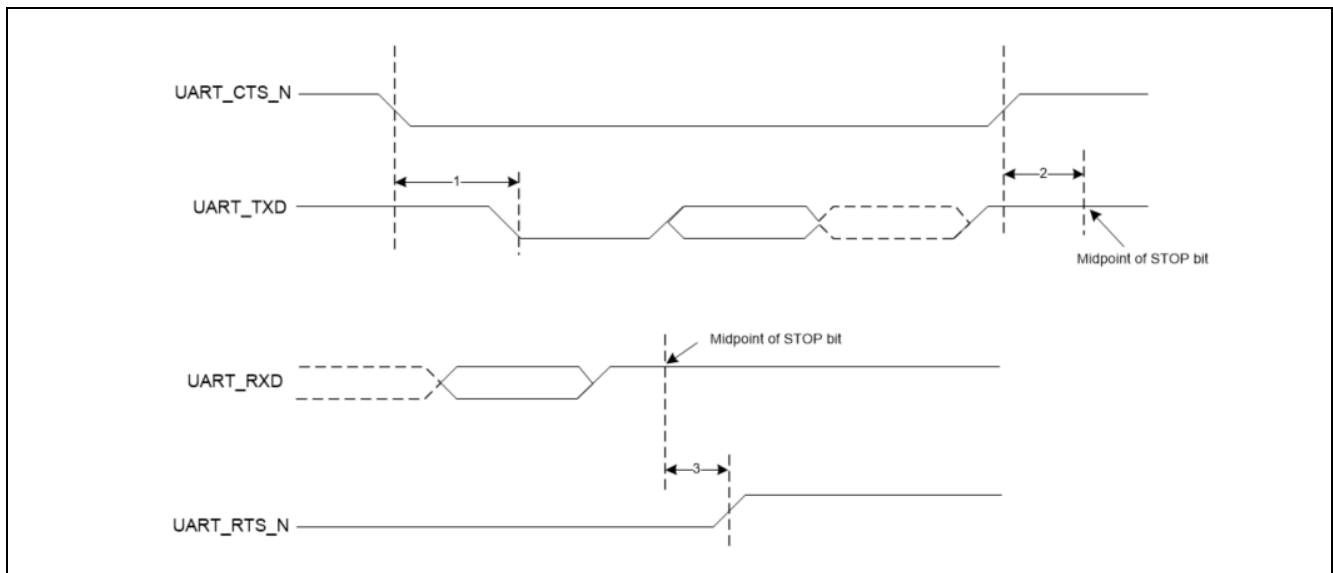
Figure 14 UART timing
