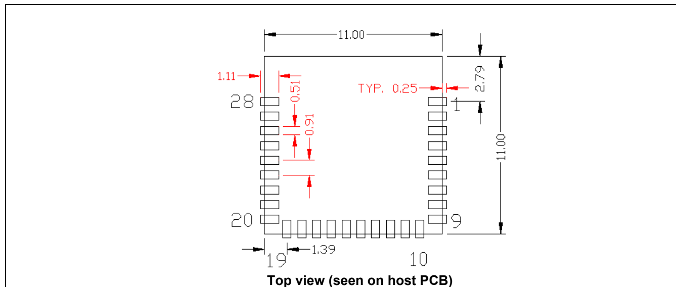
Figure 5 CYBT-4230xx-02 host layout (dimensioned)
