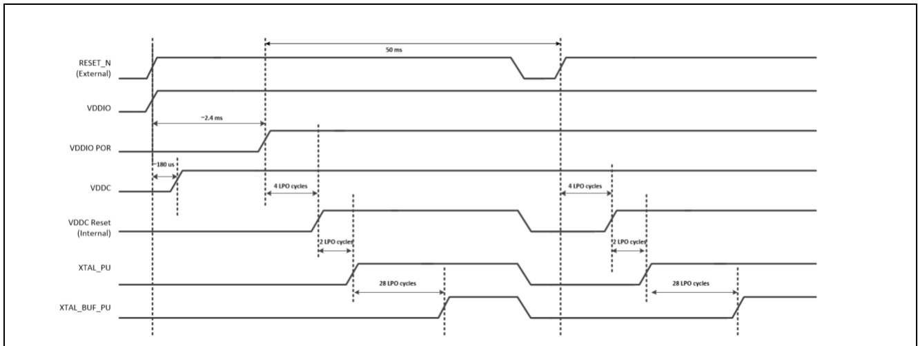
Figure 11 Reset timing
