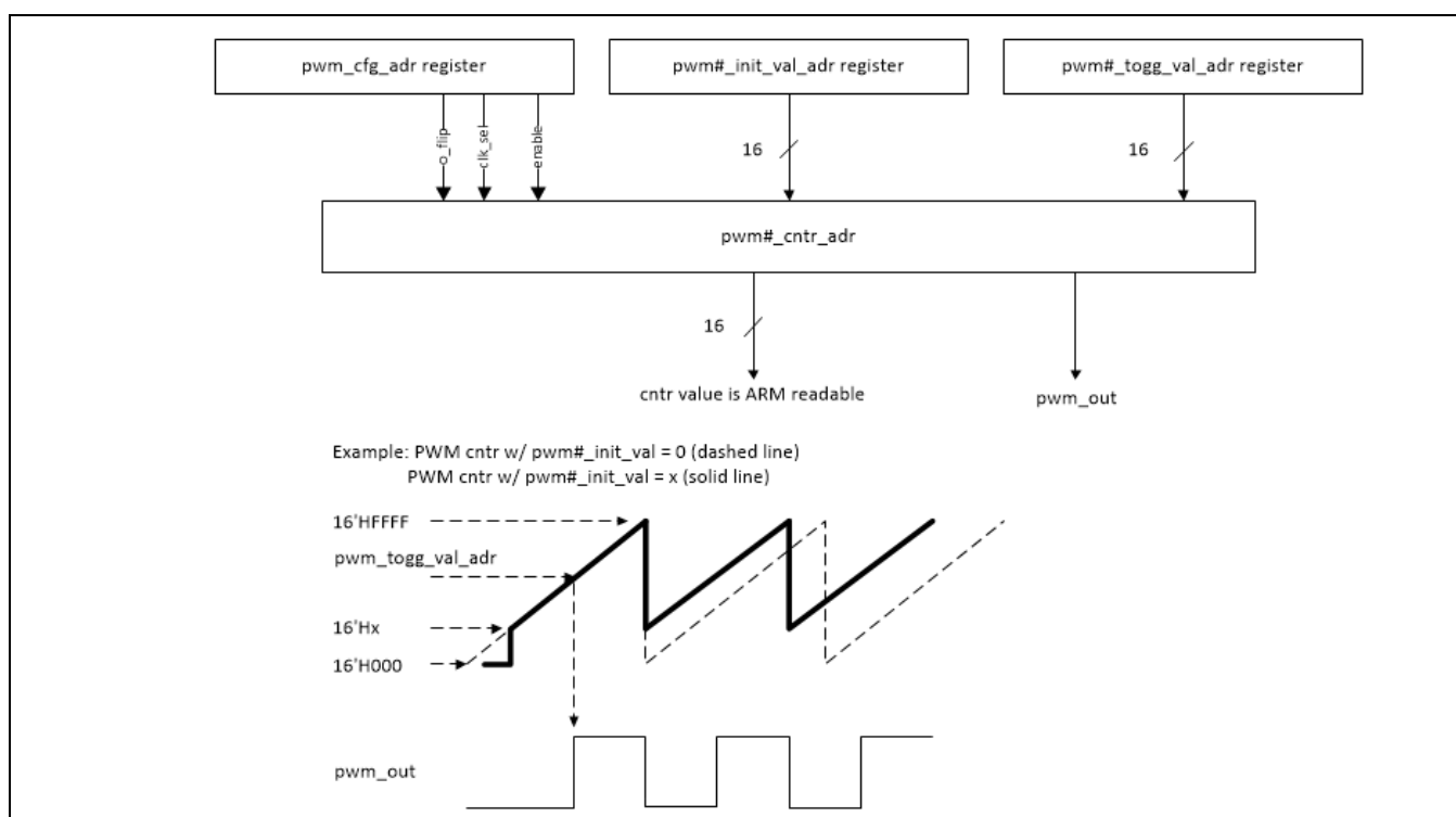
Figure 13 PWM block diagram
