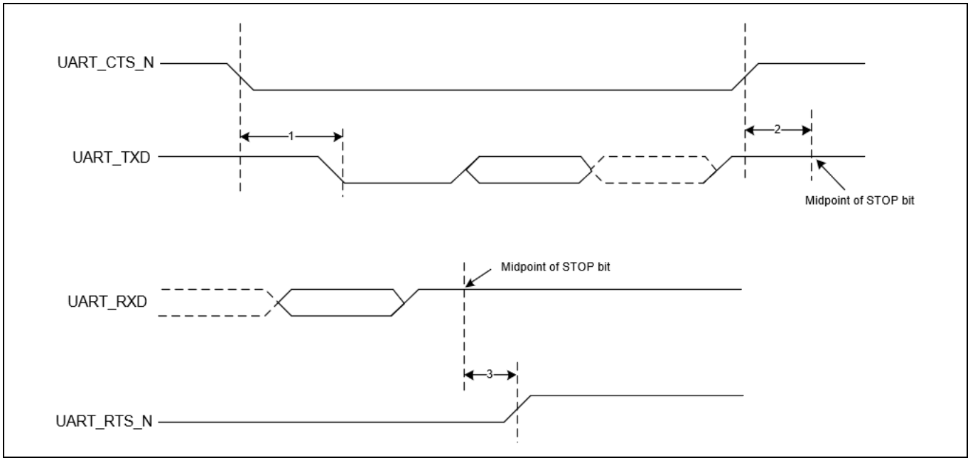
Figure 13 UART Timing
