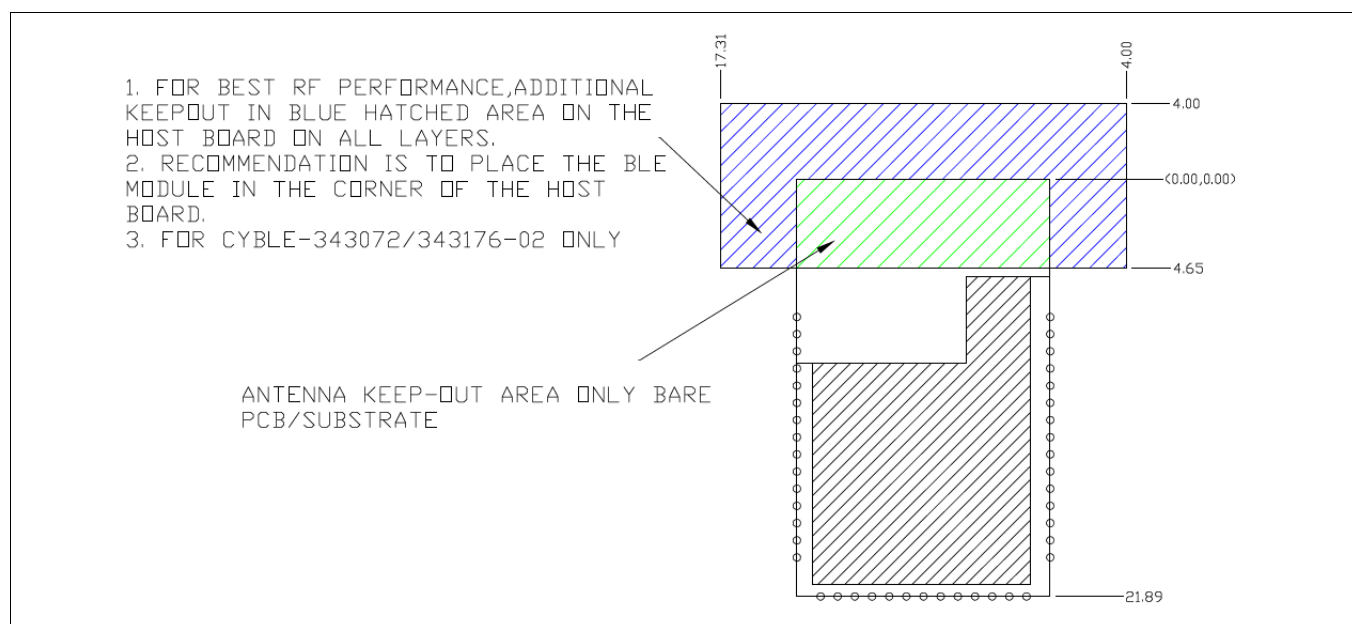
Figure 4 Recommended host PCB keepout area around the CYBLE-3x307x-02 antenna
