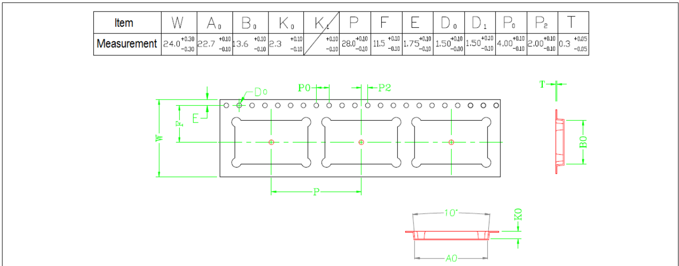
Figure 20 CYBLE-3x307x-02 tape dimensions
