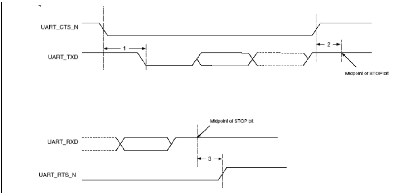
Figure 13 UART timing
