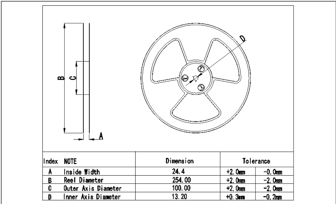
Figure 12 Reel dimensions
