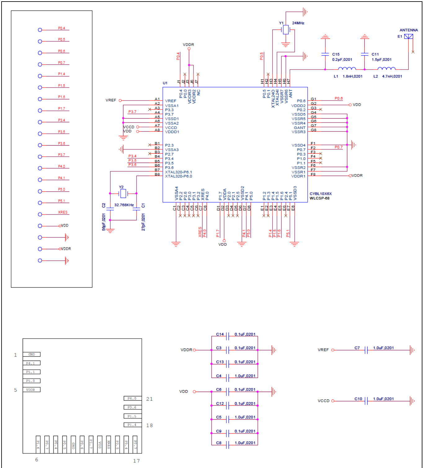
Figure 9 CYBLE-022001-00 schematic diagram
