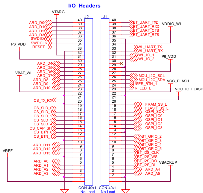
Figure 3-7. Schematics of I/O Headers (J1 and J2)
