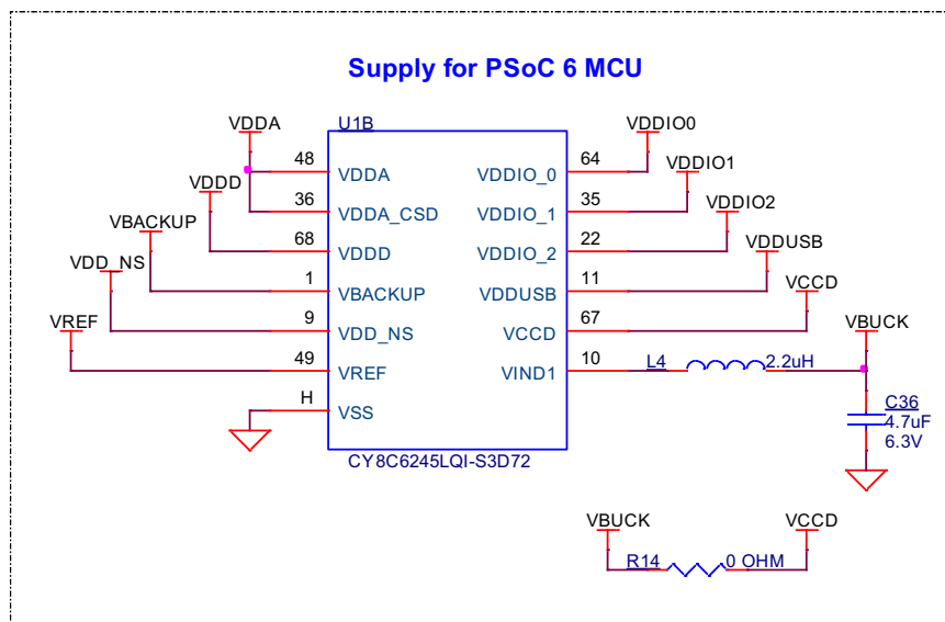
Figure 3-1. Schematics of CY8CMOD-062S3-4343W
