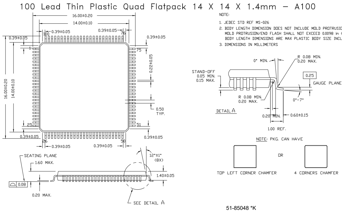
Figure 24. 100-Pin TQFP
