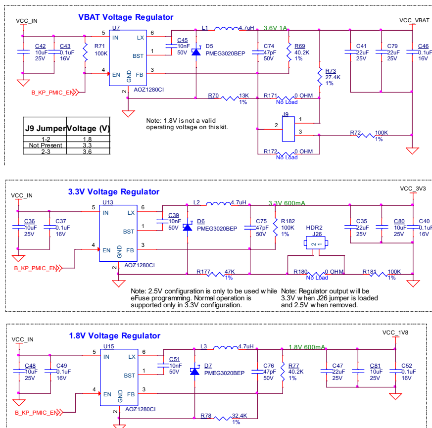
Figure 4-6. Voltage Regulators
