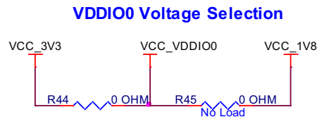
Figure 4-8. Voltage Selection
