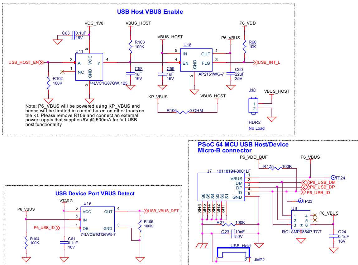
Figure 4-17. PSoC 64 MCU USB
