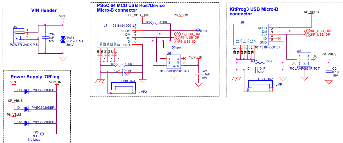
Figure 4-5. Schematics of Power Supply Input and OR'ing
