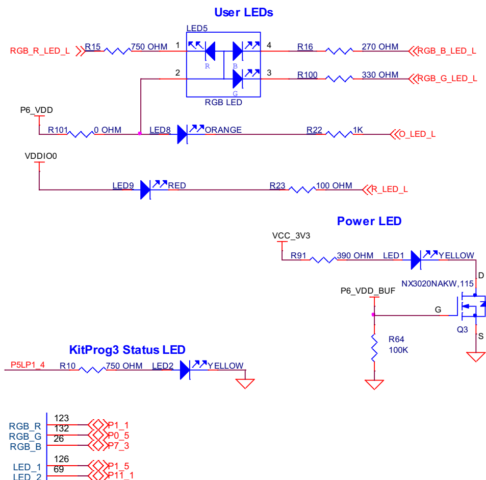
Figure 4-12. LEDs
