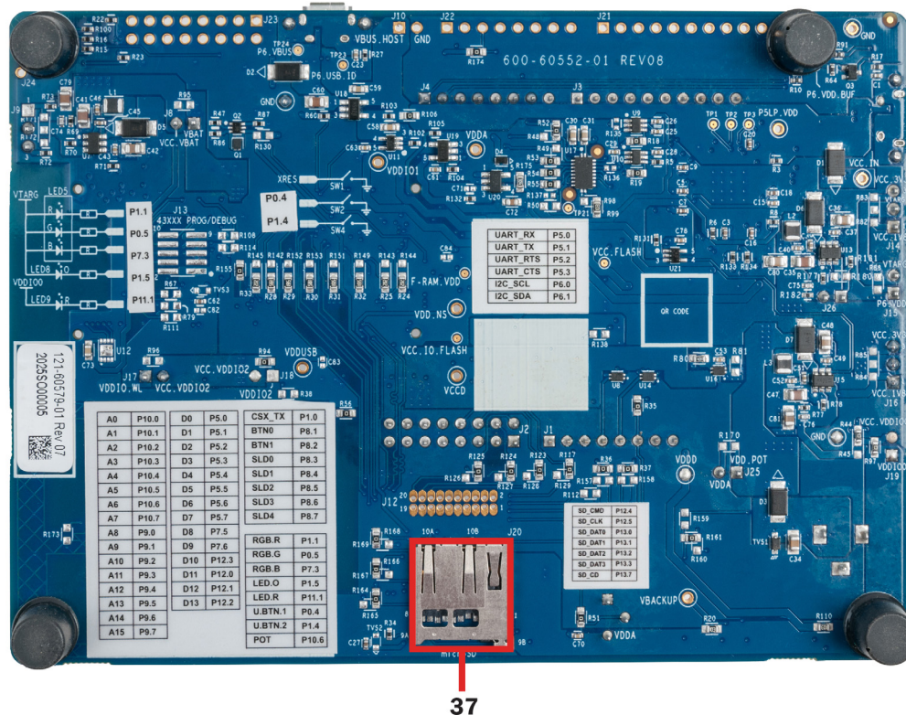
Figure 2-5. PSoC 64 Standard Secure – AWS Wi-Fi BT Pioneer Board - Bottom View
