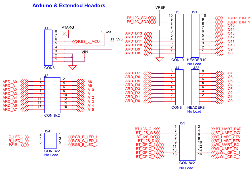
Figure 4-10. I/O Headers
