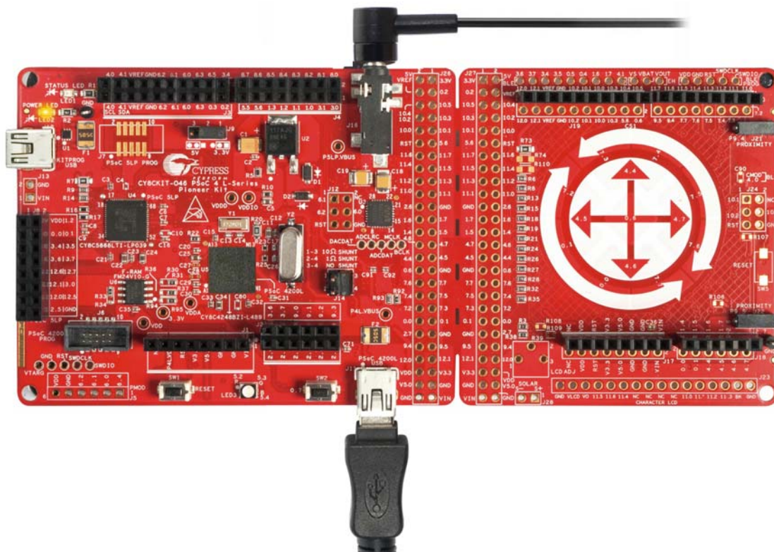
Figure 4-19. USB Audio Example Hardware Setup
