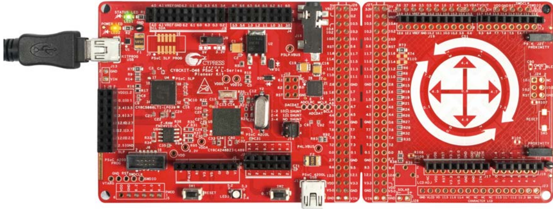
Figure 3-4. Connecting the PSoC 4 L-Series Pioneer Kit (KitProg USB) to a Computer
