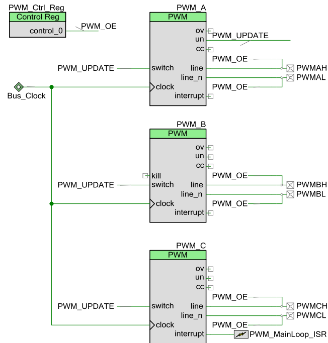
Figure 5-39. PWM Schematic
