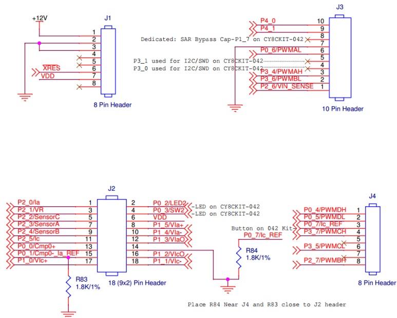
Figure 4-15. Connectors to CY8CKIT-042
