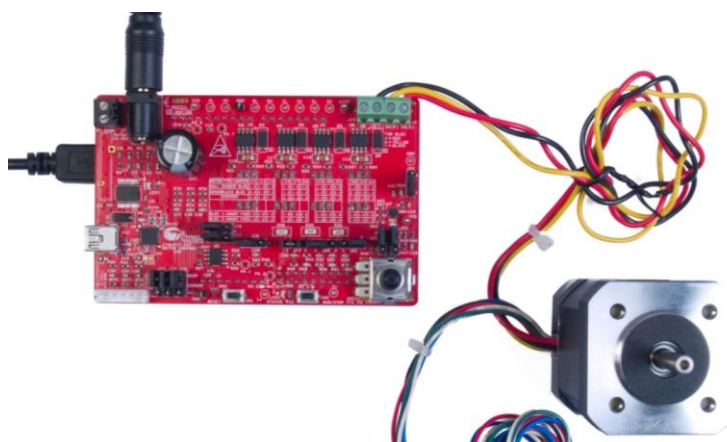
Figure 5-27. Connect Motor and Power Supply
