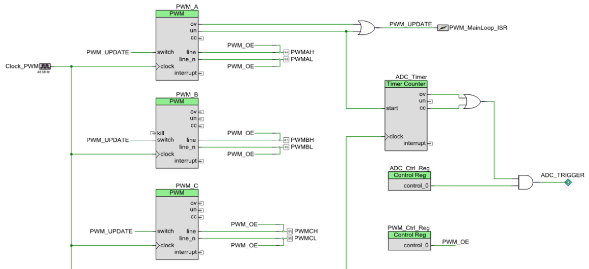
Figure 5-51. PWM Drive Schematic
