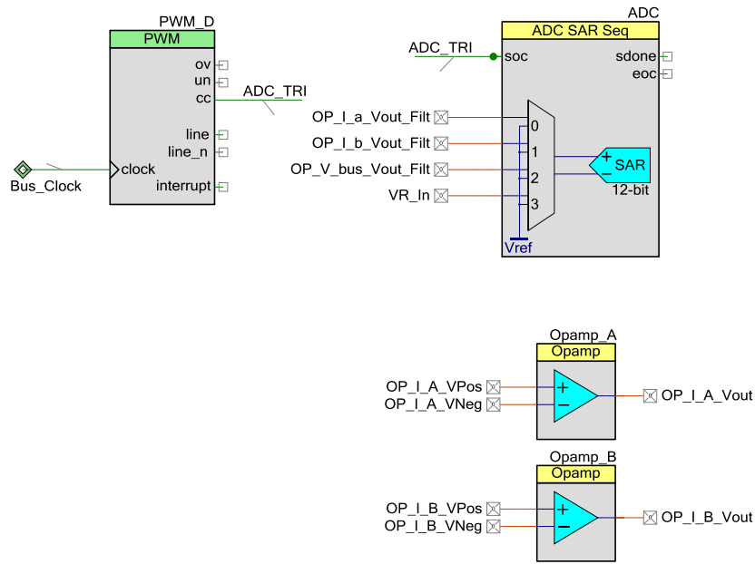
Figure 5-40. ADC Schematic
