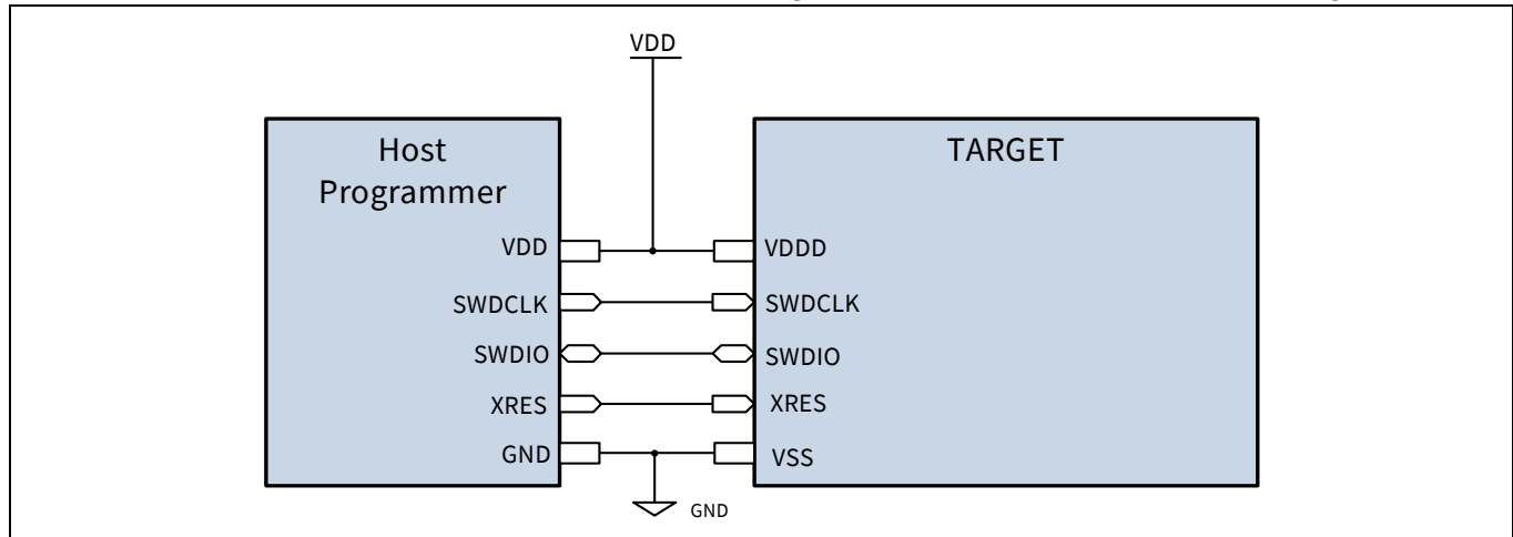
Figure 3-3. Connection schematic of programmer
