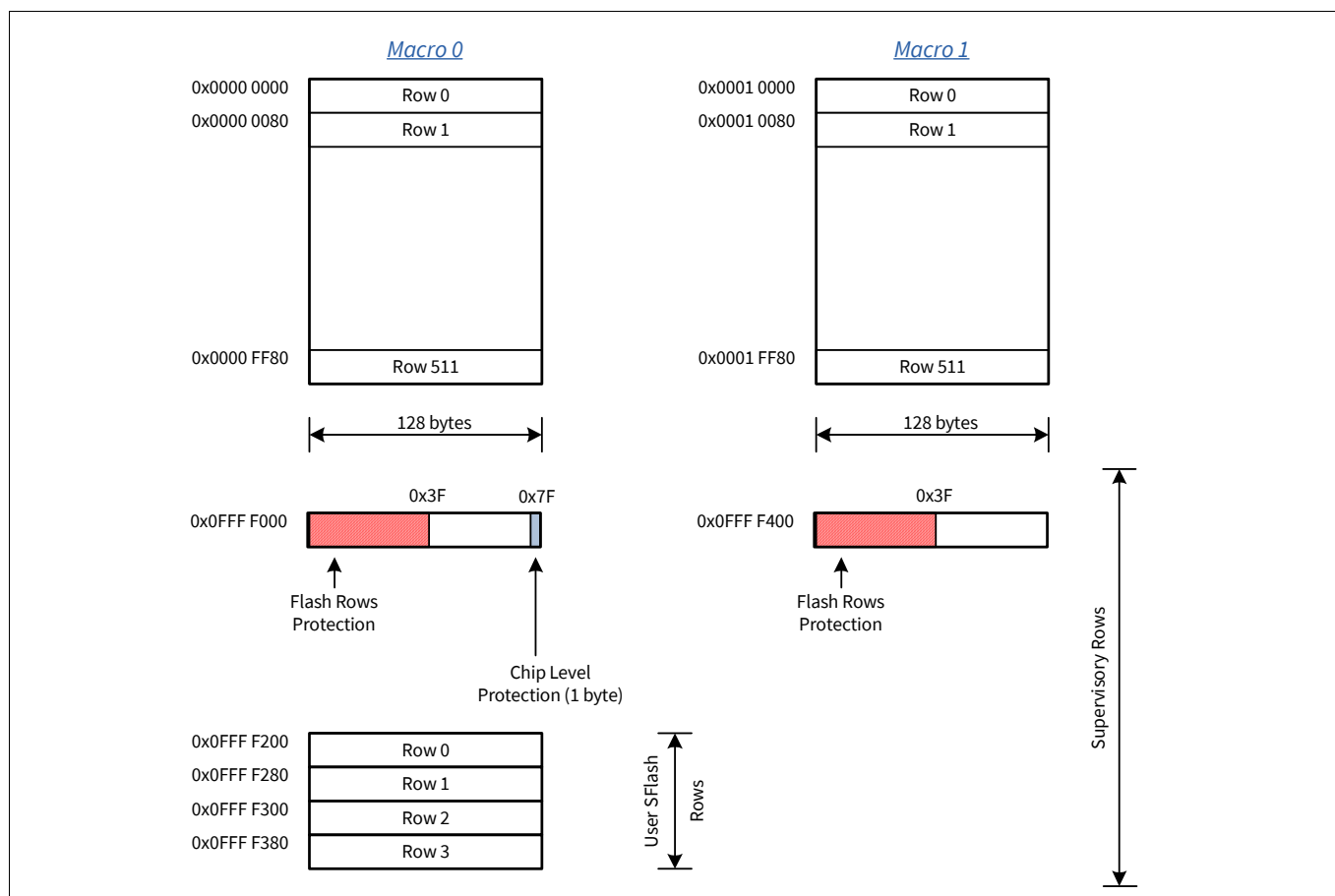
Figure 2-1. A typical nonvolatile subsystem
