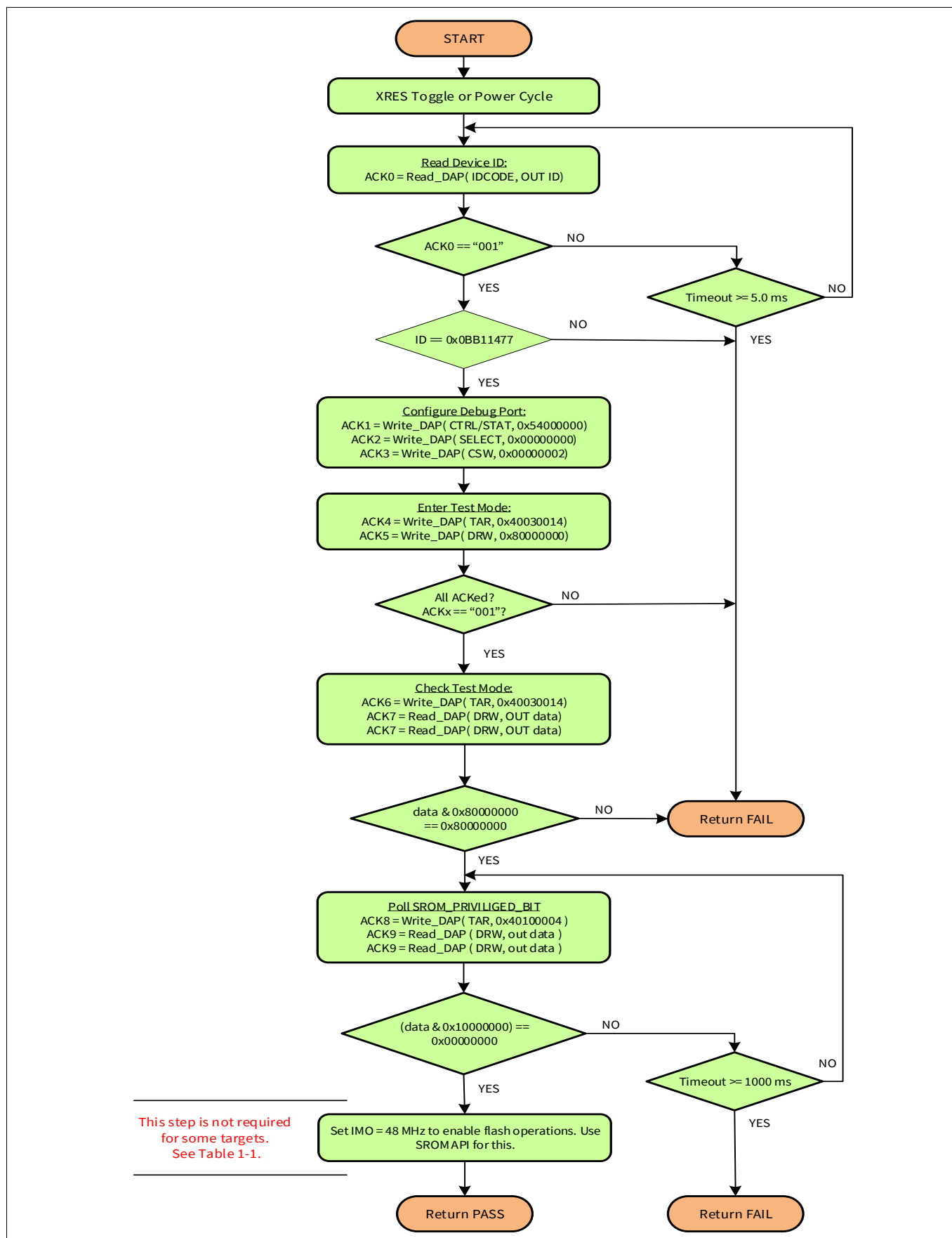
Figure 4-3. Flowchart of the “Acquire chip” step
