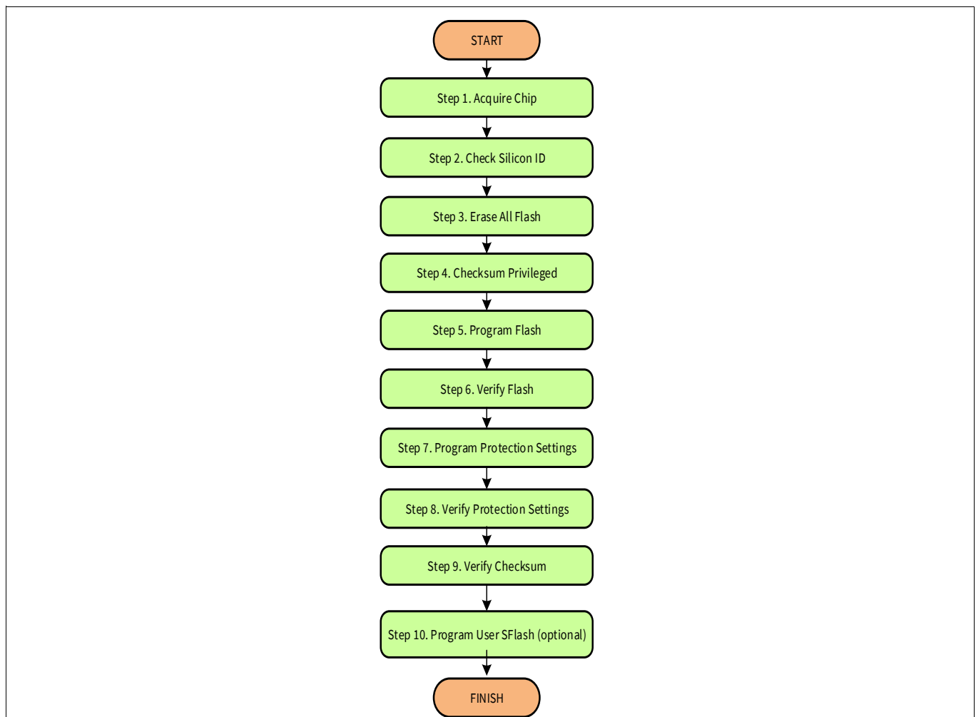
Figure 4-1. High-level programming flow of the target device
