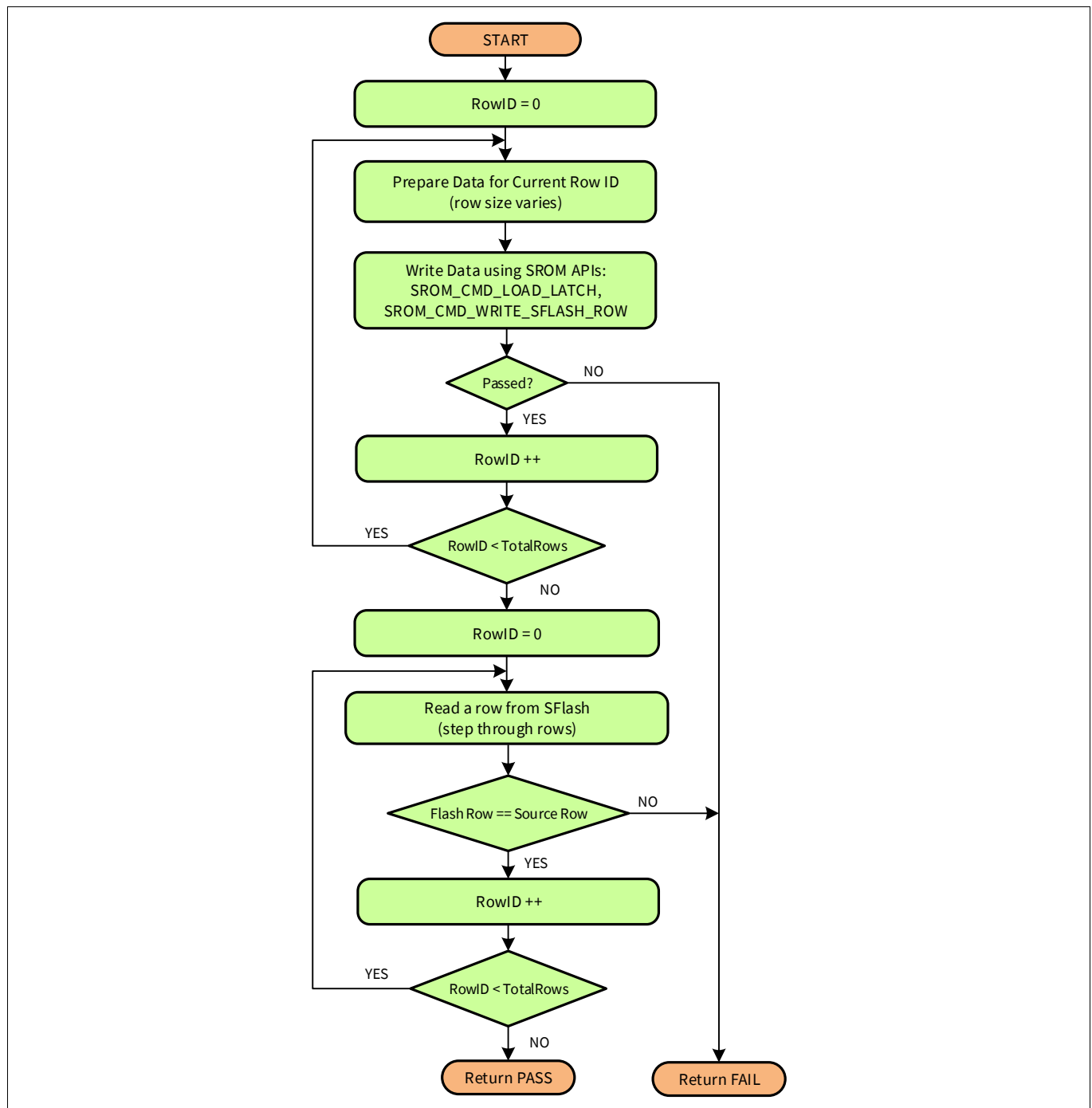
Figure 4-10. Flowchart of “Program User SFlash” step
