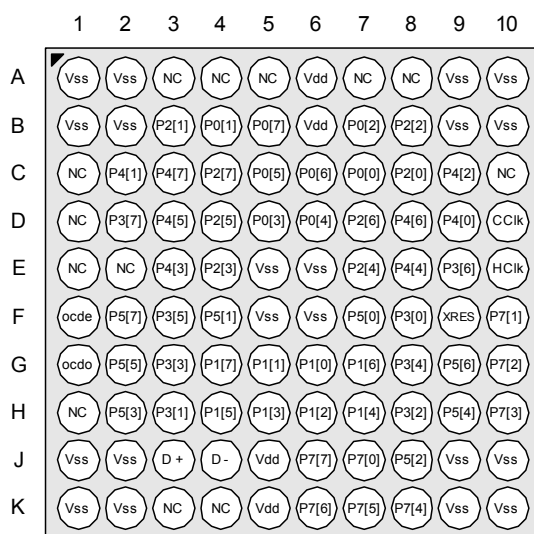
Figure 9. CY8C24094 OCD (Not for Production)
