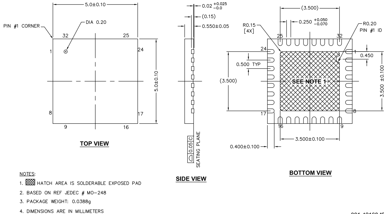
Figure 16. 32-Pin (5x5 mm) QFN
