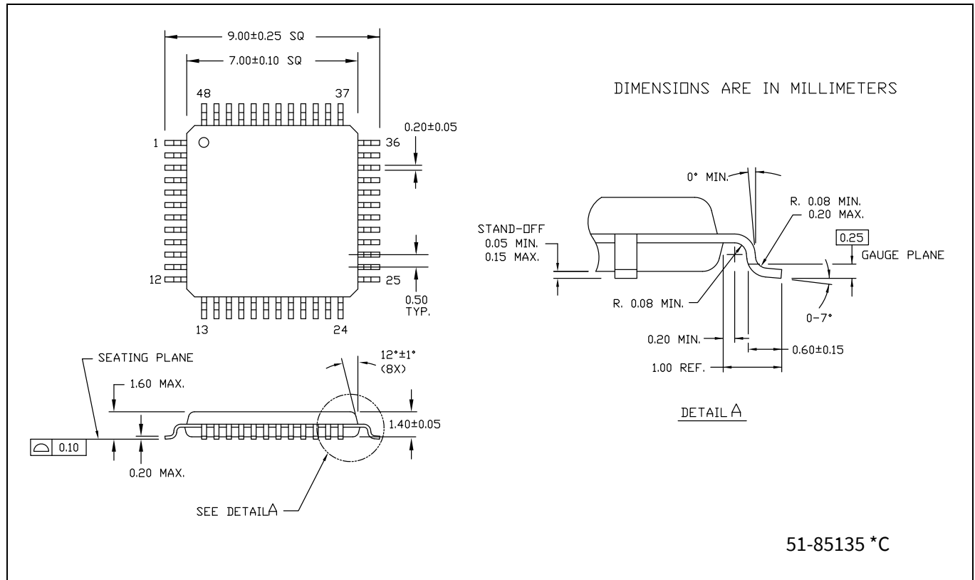
Figure 8 48-pin TQFP (7 × 7 × 1.4 mm) A48 package outline (PG-TQFP-48)
