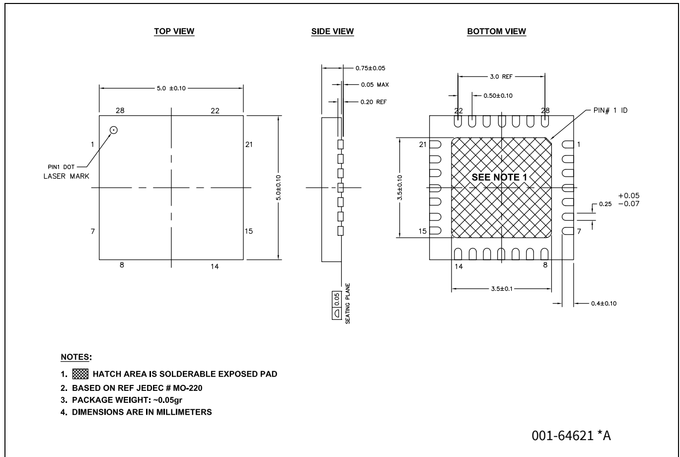
Figure 9 28-pin QFN ((5 × 5 × 0.8 mm) LT28A 3.5 × 3.5 E-Pad (Sawn)) package outline (PG-VQFN-28)
