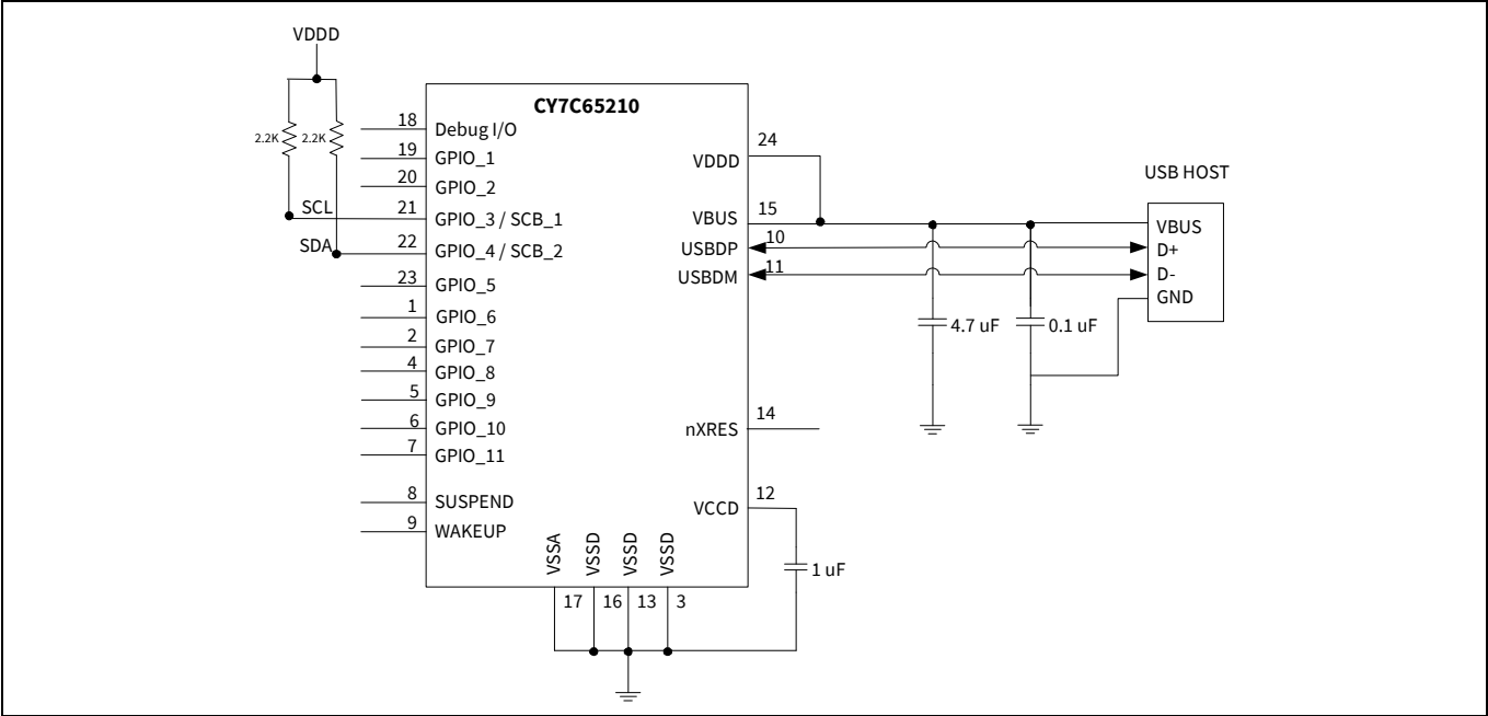
Figure 1 CY7C65210 application schematic
