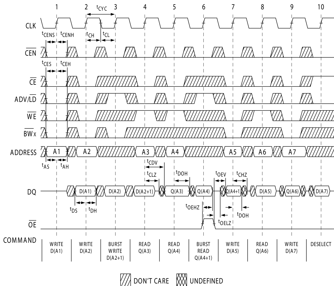
Figure 3. Read/Write Timing [21, 22, 23]
