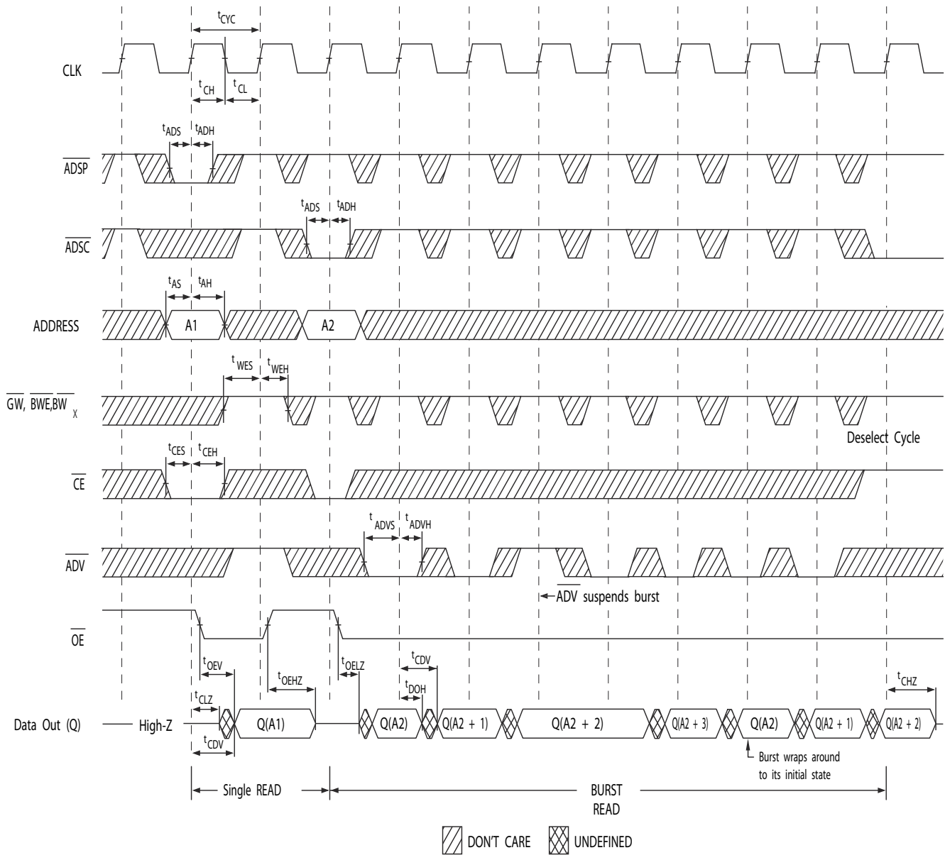
Figure 4. Read Cycle Timing [23]
