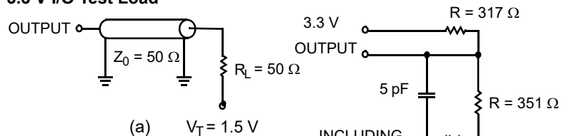
Figure 2. AC Test Loads and Waveforms
