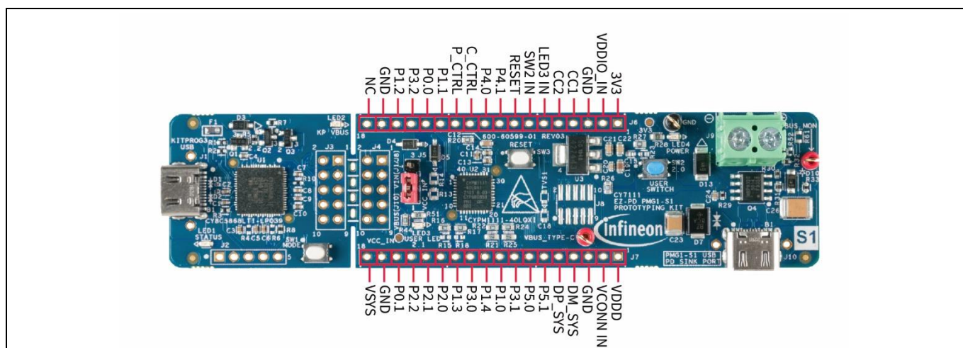
Figure 8 CY7111 prototyping kit – I/O header
