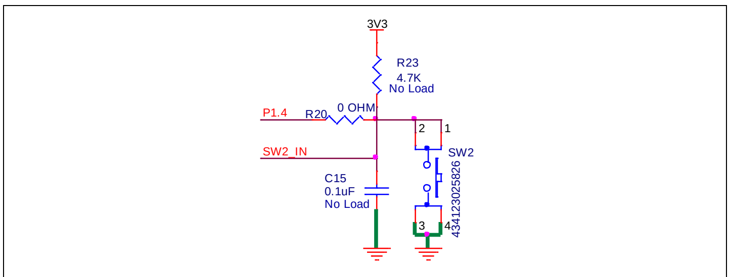
Figure 26 User button
