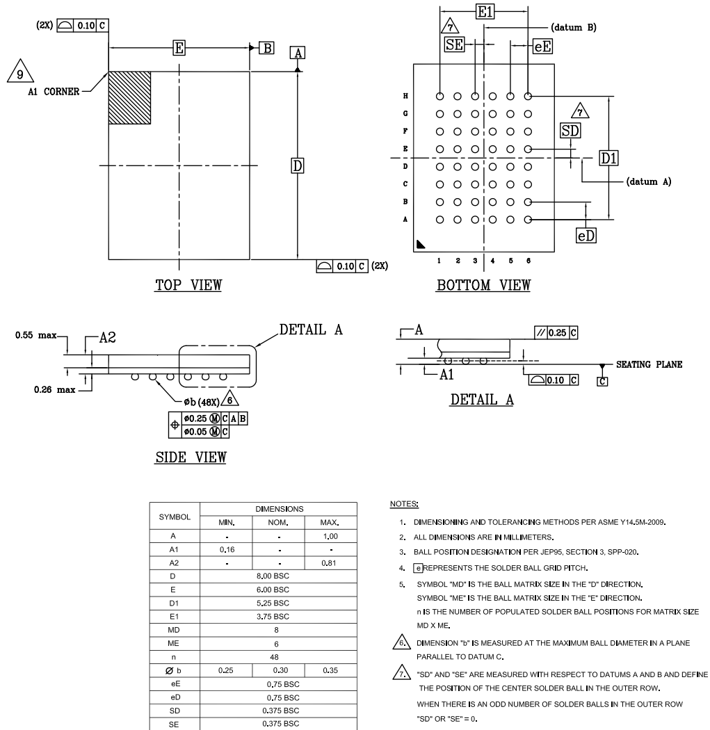
Figure 10. 48-ball VFBGA (6 × 8 × 1 mm) BV48/BZ48 Package Outline, 51-85150
