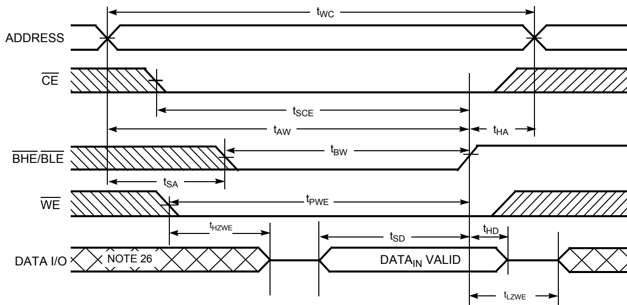
Figure 8. Write Cycle No. 4 ( \overline{BHE/BLER} Controlled, \overline{OE} LOW) [25]
