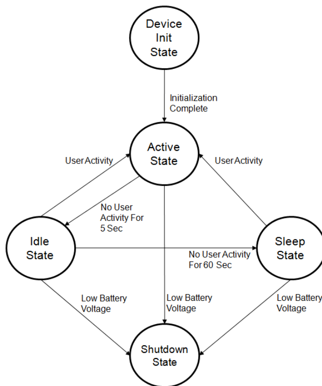
Figure 5-1. State Machine for Touch Mouse
