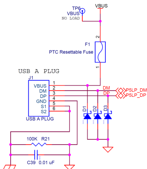
Figure 4-25. USB Circuitry
