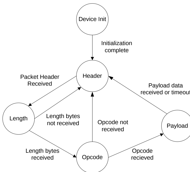
Figure 5-52. UART Packet State Machine
