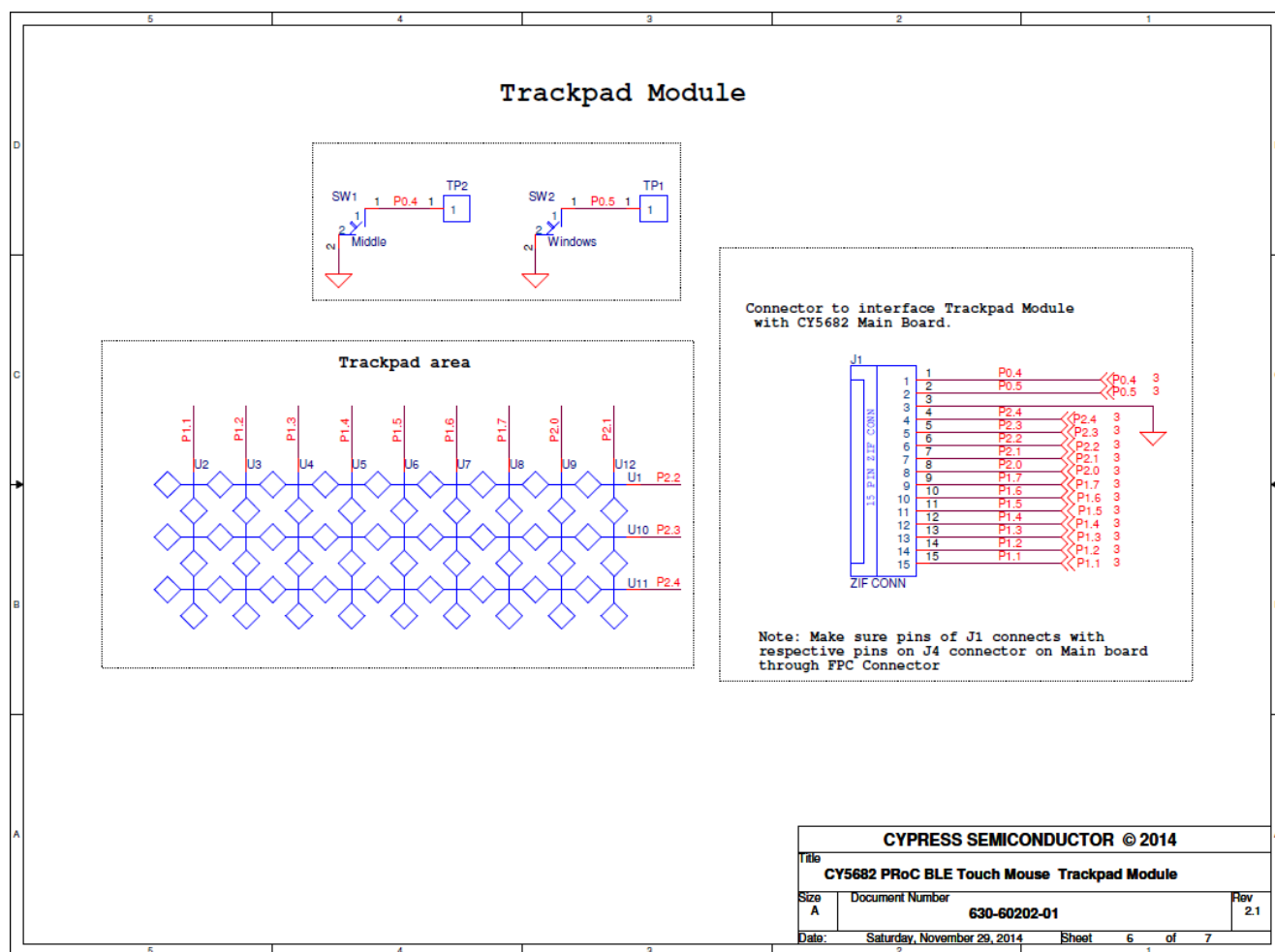
Figure A-5. Trackpad Module Schematic
