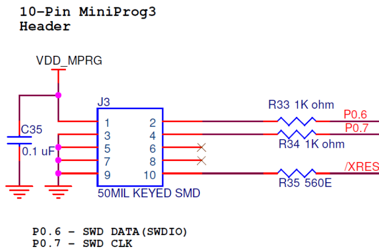
Figure 4-11. SWD Debug Header
