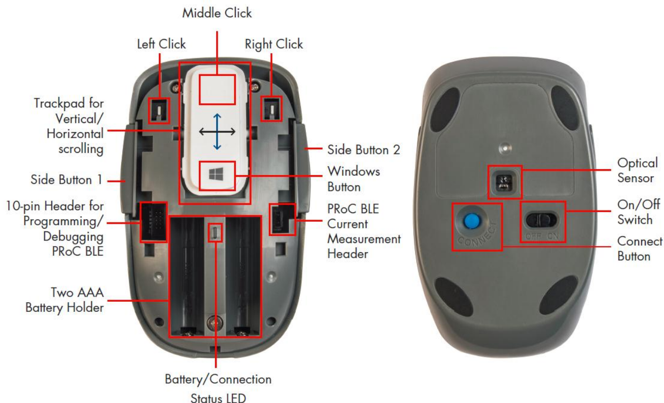
Figure 1-2. PRoC BLE Touch Mouse Features
