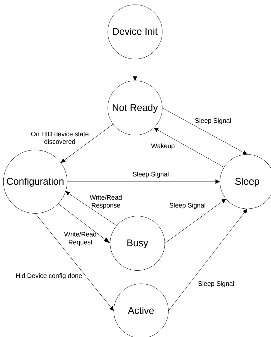
Figure 5-41. State Machine for PProC BLE Firmware
