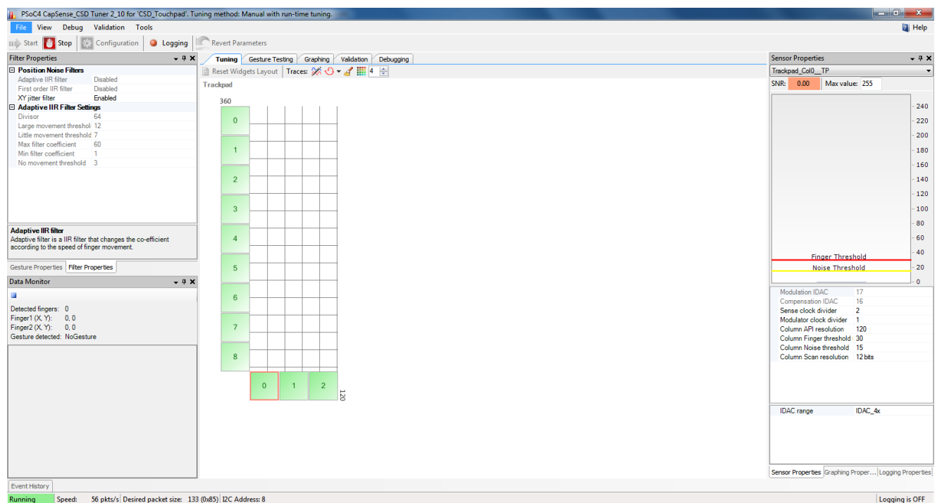
Figure 5-24. Tuner Tool
