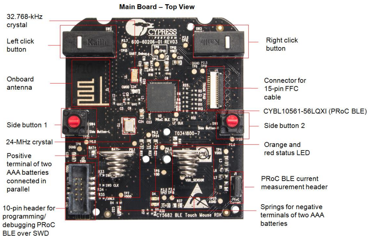
Figure 4-1. CY5682 PProC BLE Touch Mouse Main Board and Trackpad Module Top View (with FFC Cable)
