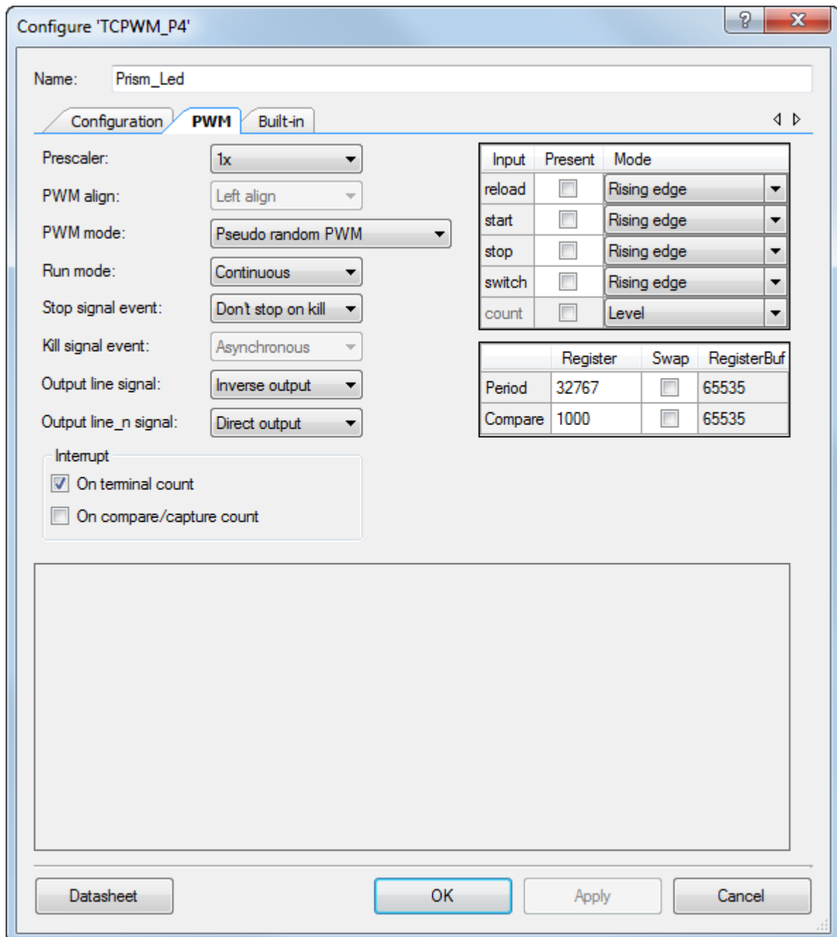
Figure 5-35. PWM Tab of TCPWM Component
