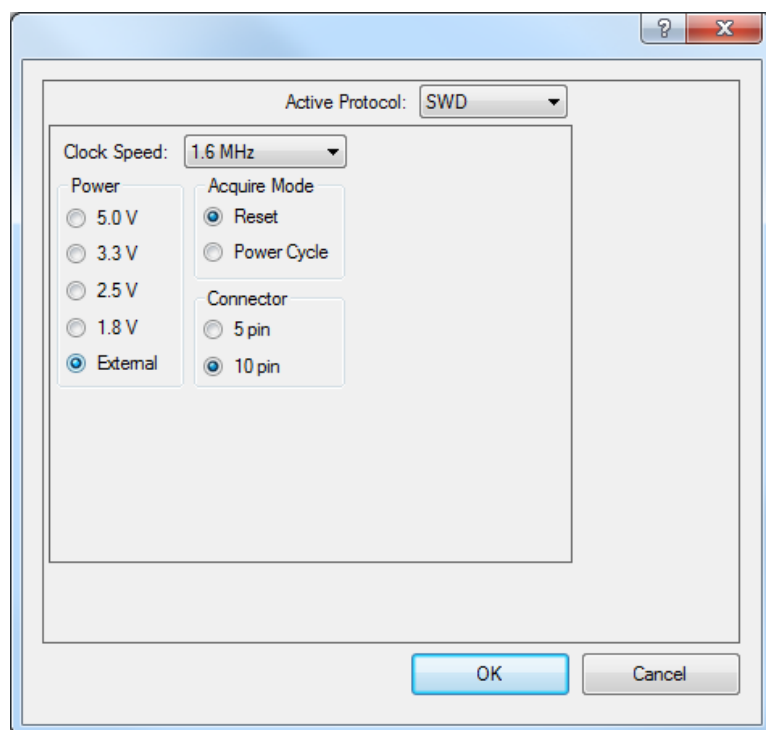
Figure 3-7. Port Settings
