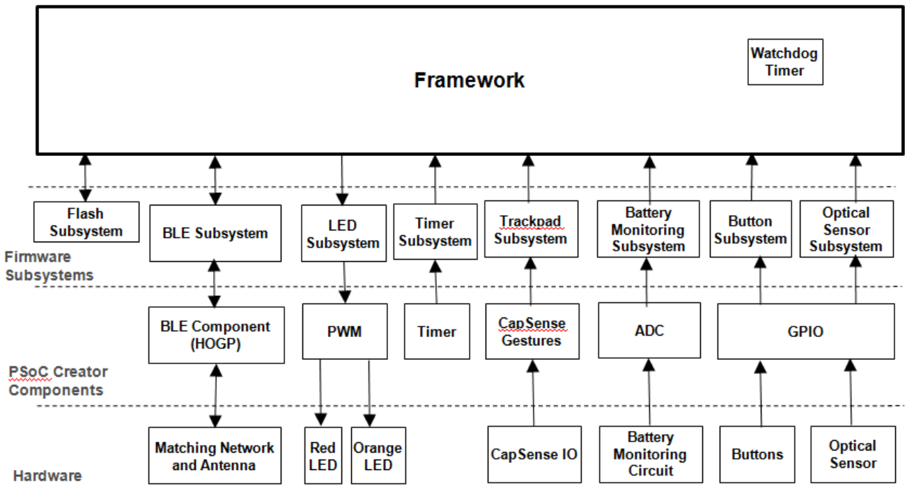
Figure 5-2. Firmware Architecture
