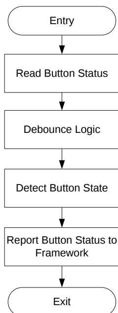
Figure 5-27. Button Subsystem Flow Chart
