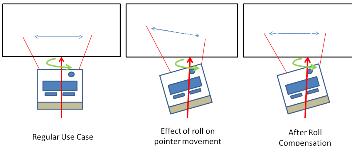
Figure 5-32. Roll Compensation
