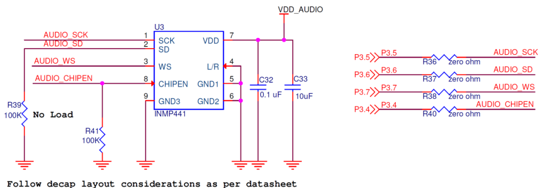
Figure 4-19. Audio Circuit
