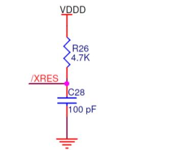
Figure 4-10. Reset Circuit
