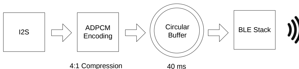
Figure 5-48. Firmware Data Flow for Audio Feature
