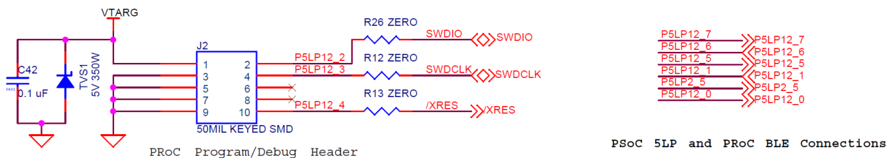
Figure 4-24. SWD Debug Header
