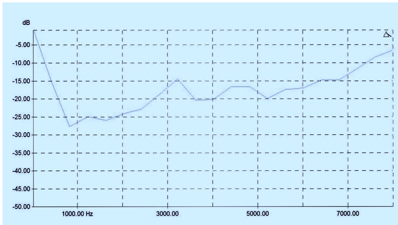
Figure 5-50. SNR for Voice Data Processed Using ADPCM Coding
