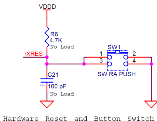
Figure 4-23. Reset Circuit
