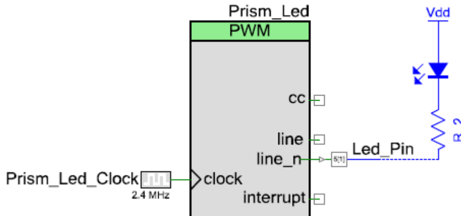
Figure 5-69. PWM Component
