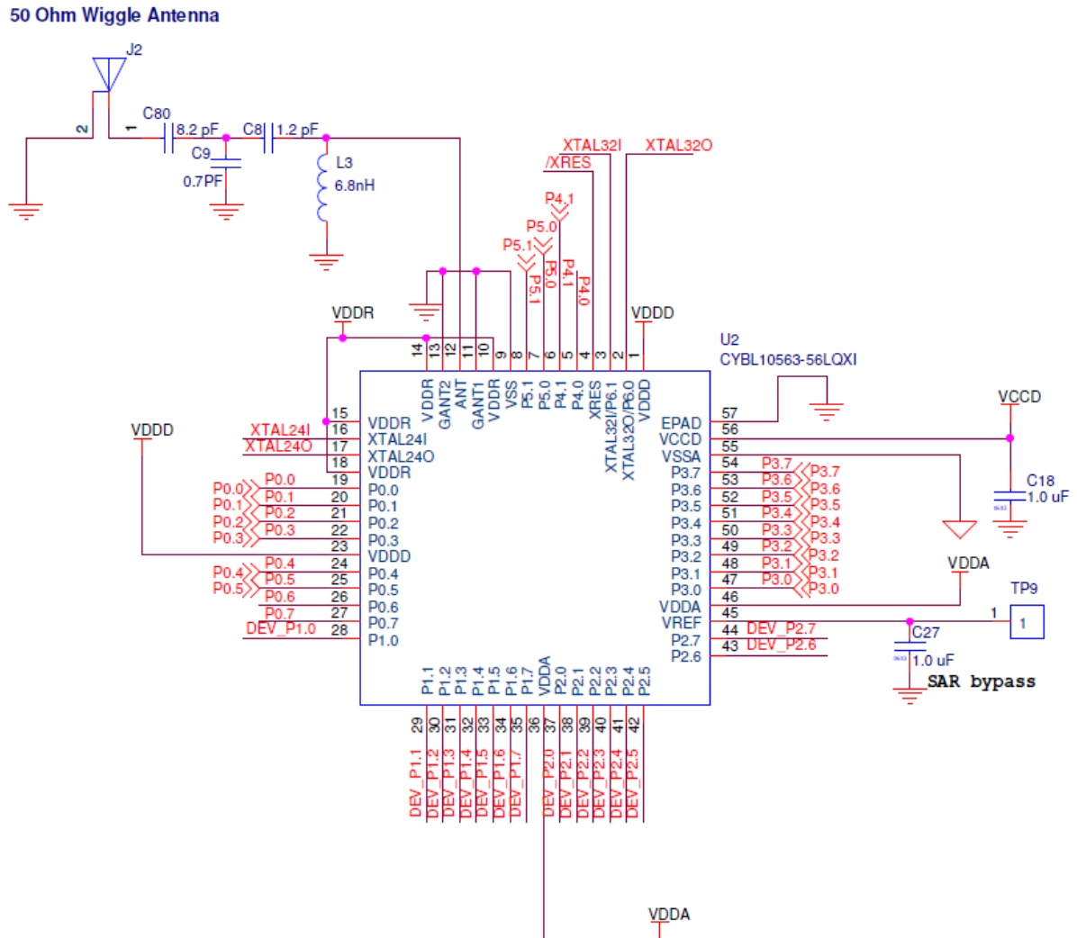
Figure 4-12. PProC BLE Connections
