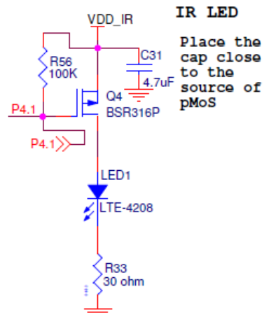
Figure 4-15. IR LED Circuitry
