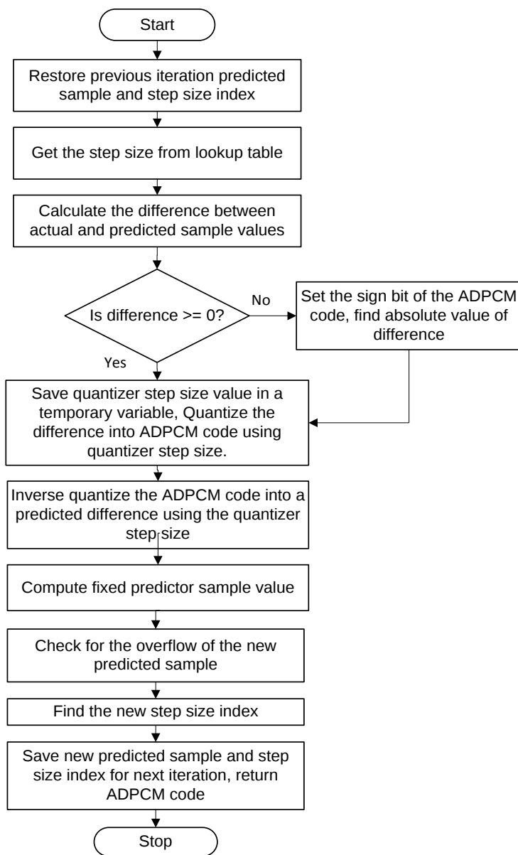
Figure 5-51. ADPCM Algorithm Flow Chart
