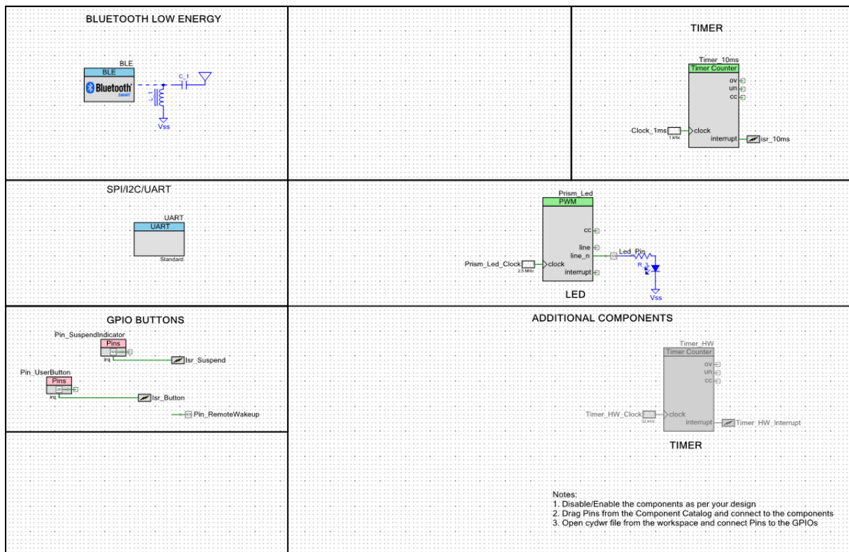
Figure 5-73. Schematic View of BLE HID CySmart Dongle Firmware (PSoC BLE)
