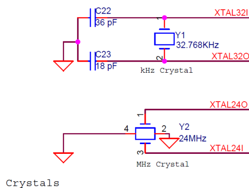
Figure 4-22. Crystal Circuit
