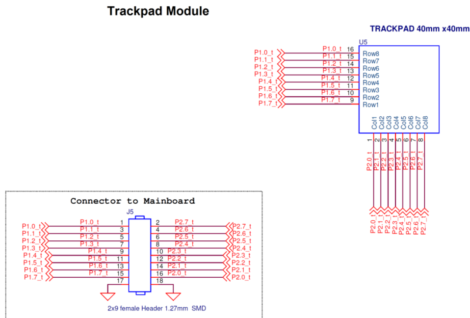
Figure 4-20. Trackpad Circuit
