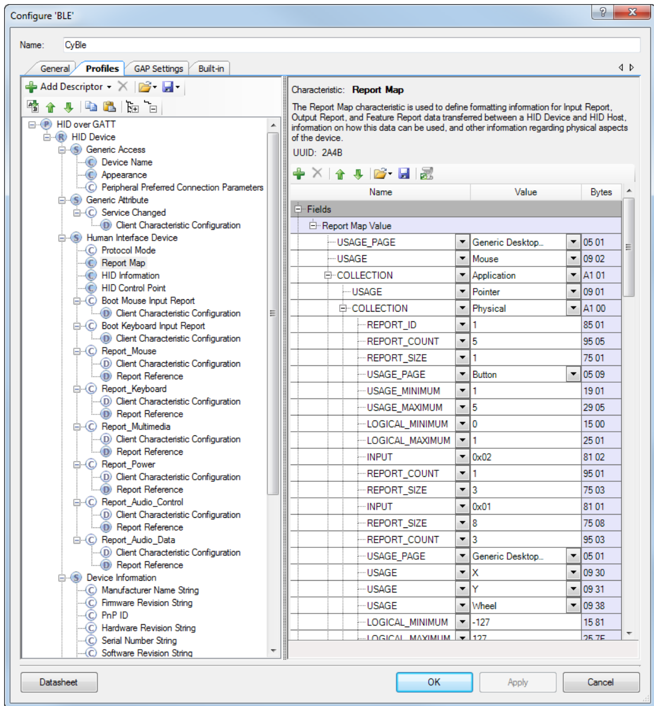
Figure 5-7. Profiles Tab of BLE Component
