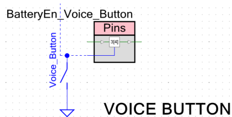
Figure 5-35. cy_pins Component for Button Module
