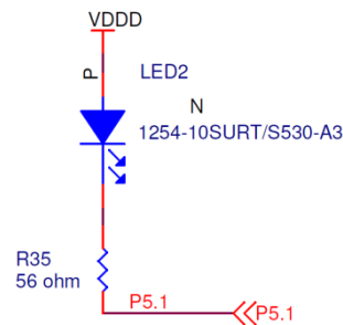
Figure 4-13. LED
