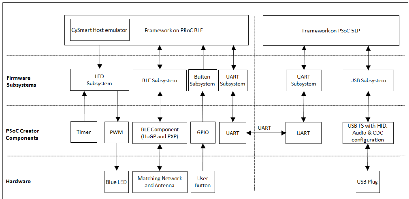
Figure 5-72. PSoC BLE Firmware Architecture for CySmart USB Dongle
