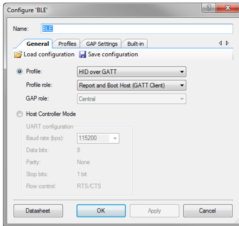
Figure 5-81. BLE Component General Configuration
