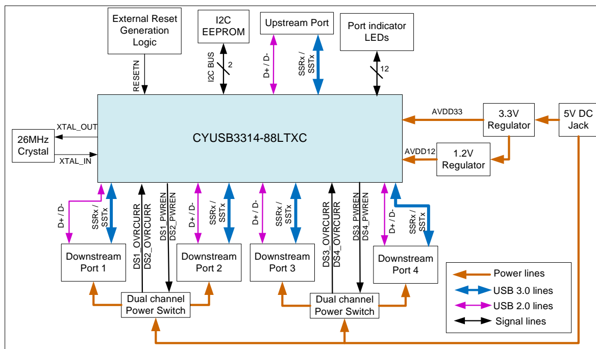
Figure 5-11. CY4603 Hardware Block Diagram
