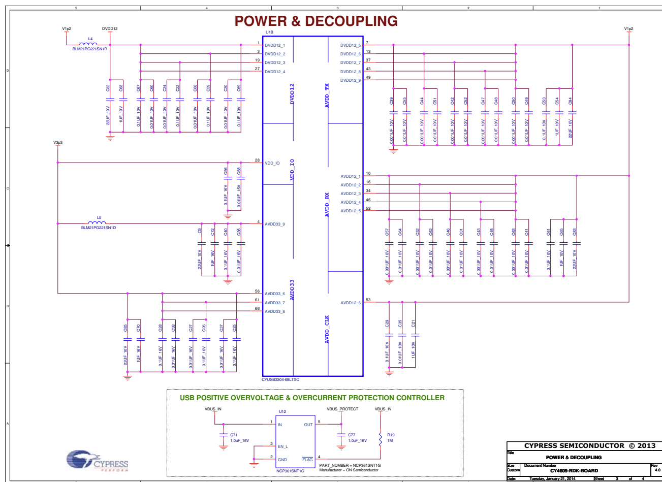
Figure A-2. Overvoltage, Overcurrent Protection, and Decoupling Capacitors
