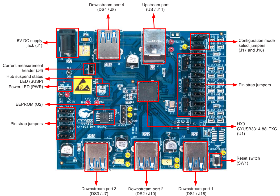
Figure 3-4. CY4603 Board (Top Side)
