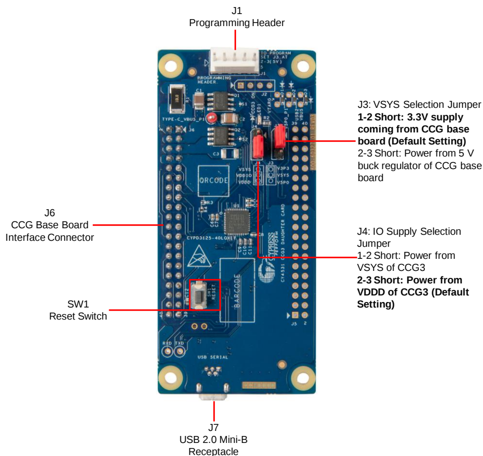
Figure 3-5: CCG3 Daughter Card Connectors/Jumper Settings
