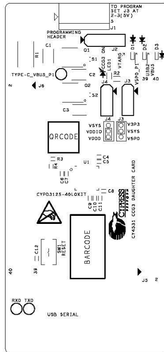
600-60327-01 REV03 PRIMARY SILKSCREEN
