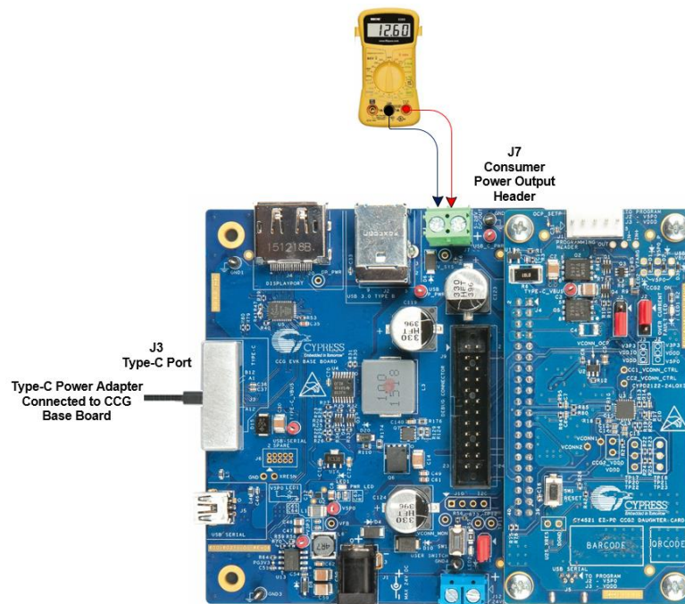
Figure 5-6: Setup of Dead Battery Demo Using CY4521 EZ-PD CCG2 EVK
