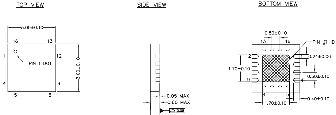
Figure 18. 16-pin QFN ( 3 \times 3 \times 0.6 mm) LQ16A 1.7 \times 1.7 E-Pad (Sawn) Package Outline, 001-87187
