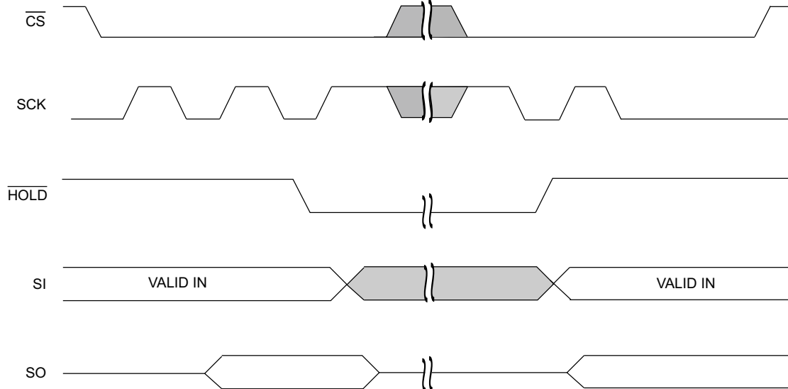
Figure 12. HOLD Operation [2]
