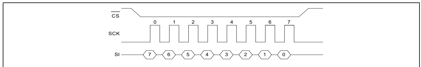
Figure 4 SPI mode 0
