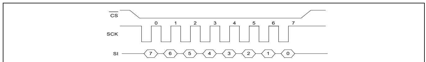
Figure 5 SPI mode 3
