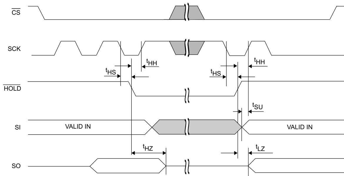
Figure 17. \overline{\text{HOLD}} Timing
