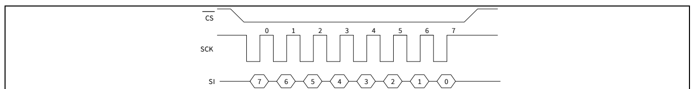
Figure 5 SPI mode 3
