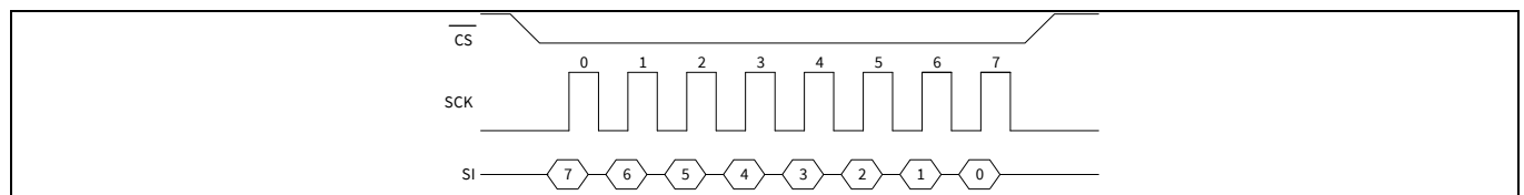
Figure 4 SPI mode 0
