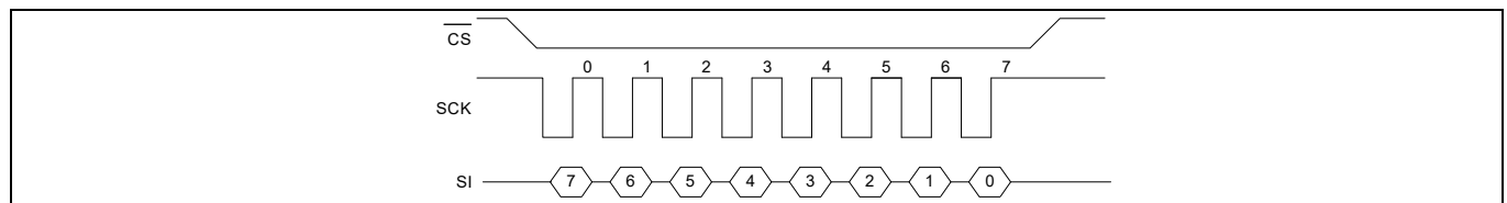
Figure 5 SPI mode 3
