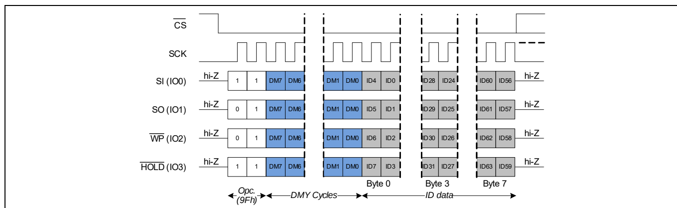
Figure 89 Read device ID (RDID) in QPI mode
