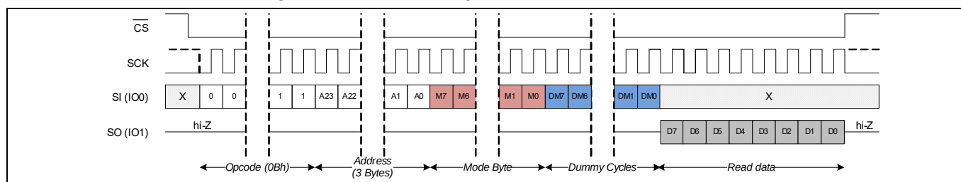
Figure 55 FAST_READ in SPI mode
