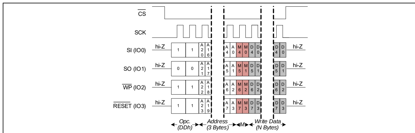
Figure 46 DDR fast write (DDR_FAST_WRITE) in QPI mode
