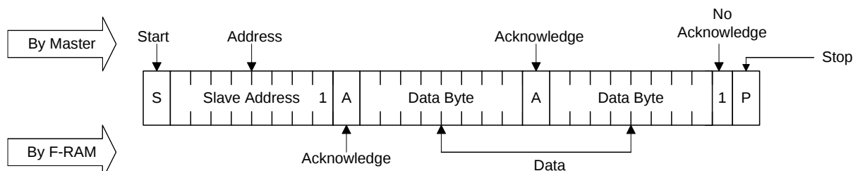
Figure 10. Sequential Read
