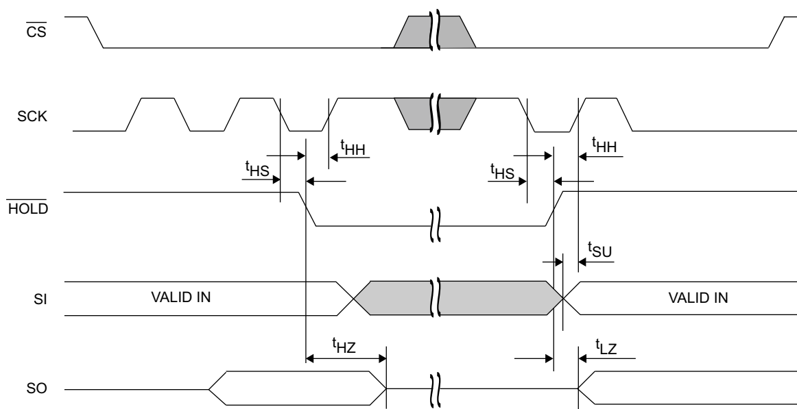
Figure 14. \overline{\text{HOLD}} Timing
