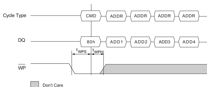
Figure 22. Write Protect Enable Timing
