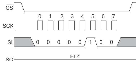
Figure 9. WRDI Instruction
