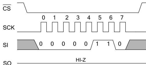
Figure 8. WREN Instruction
